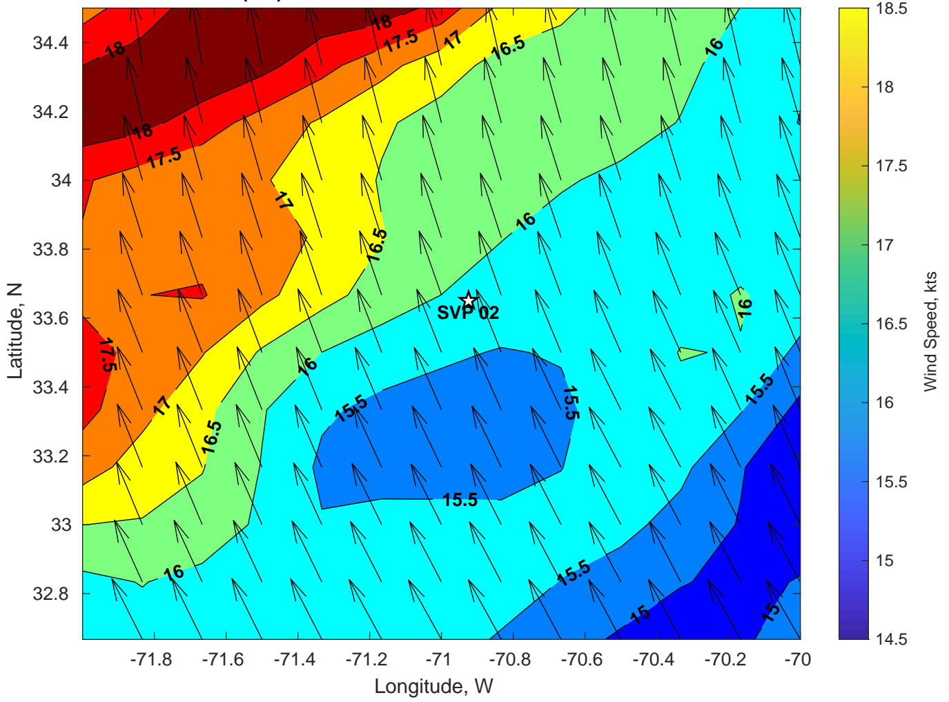
Winds (kts) for SVP 02 at 13-Jul-2024 06:00:00
