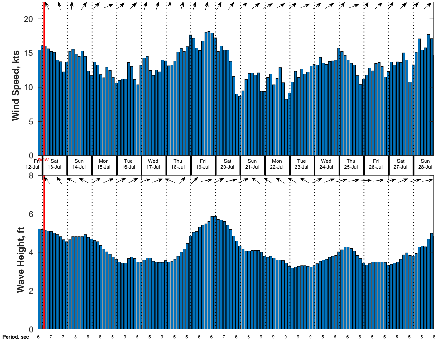
Wind & Wave Forecast for SVP 02 from 12-Jul-2024 19:00:00 to 28-Jul-2024 19:00:00
