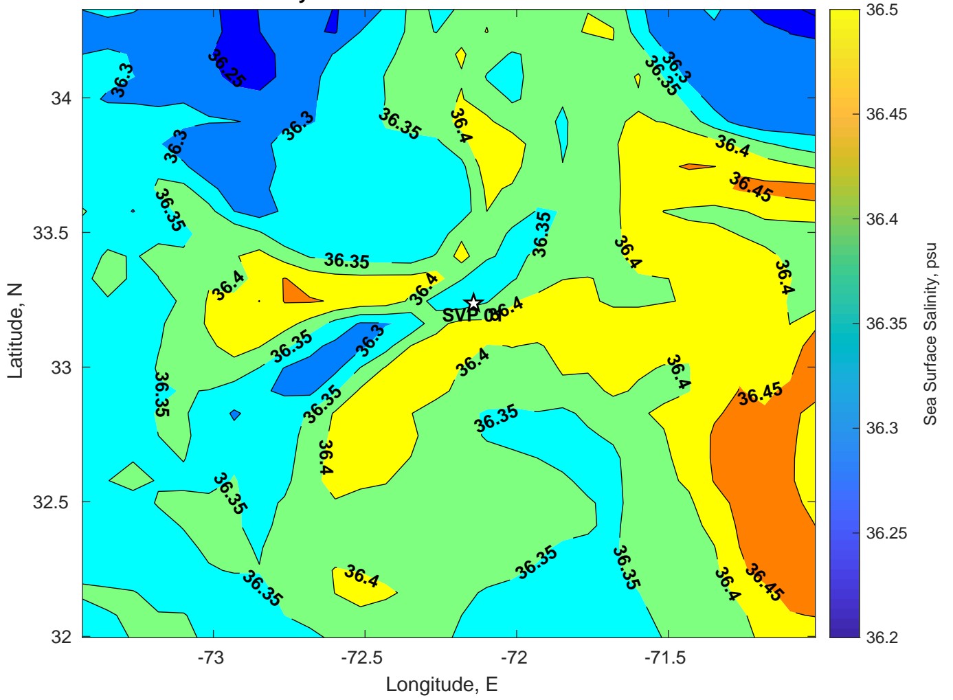
Surface Salinity for SVP 01 at 14-Jul-2024 00:00:00
