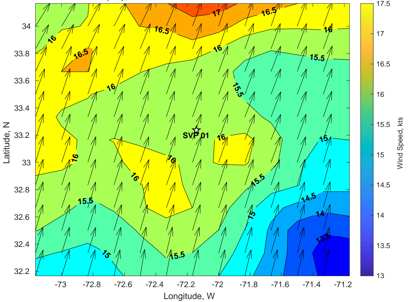
Winds (kts) for SVP 01 at 14-Jul-2024 06:00:00
