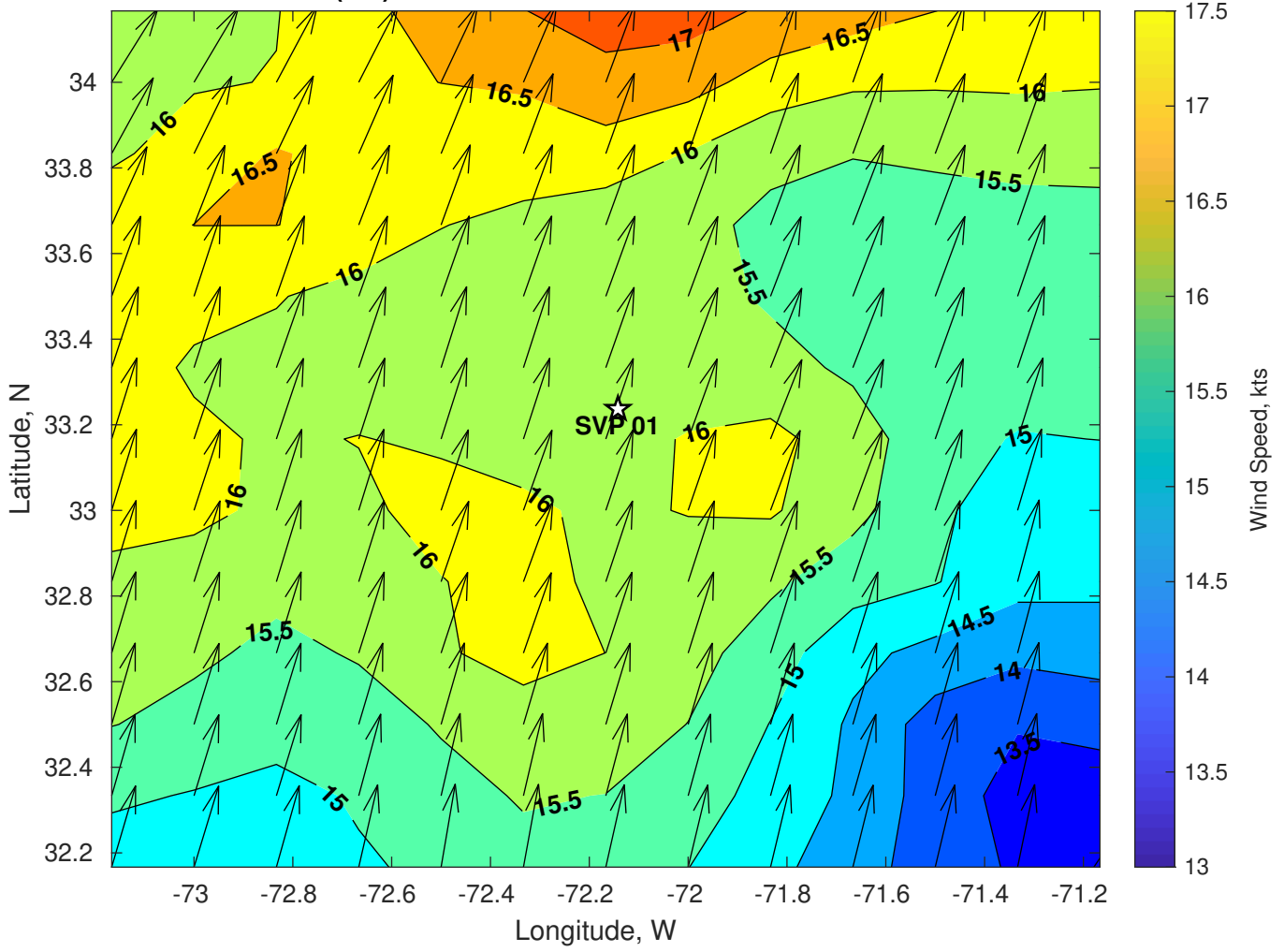
Winds (kts) for SVP 01 at 14-Jul-2024 06:00:00
