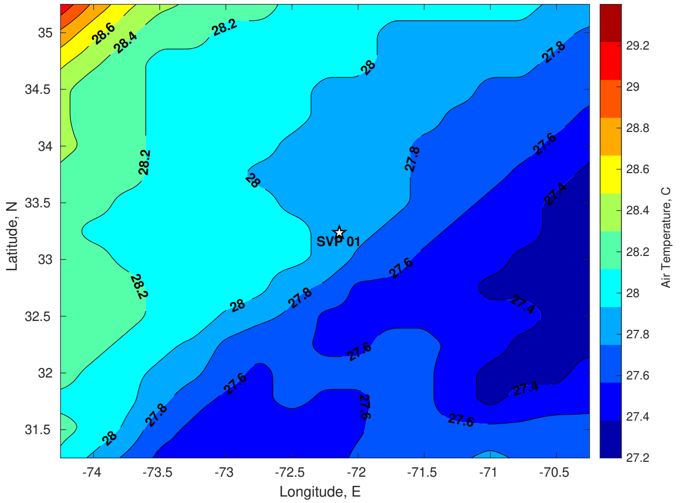
Air Temperature (C) for SVP 01 at 14-Jul-2024
