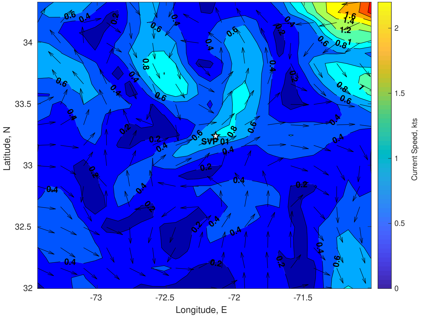
Surface Currents for SVP 01 at 14-Jul-2024 00:00:00
