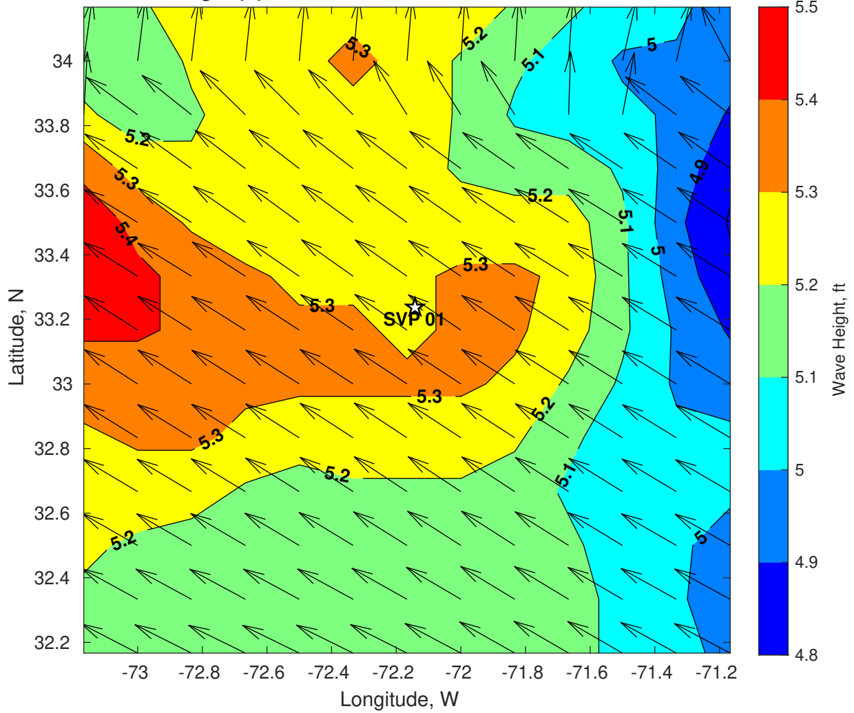
Wave Height (ft) for SVP 01 at 14-Jul-2024 06:00:00
