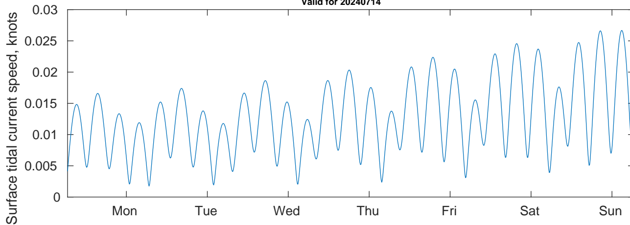
Tidal Currents and Heights for SVP 01 at 20240714
