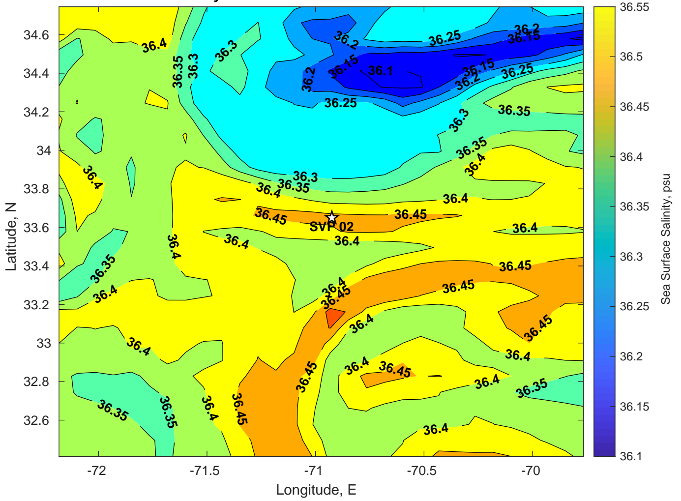
Surface Salinity for SVP 02 at 14-Jul-2024 00:00:00
