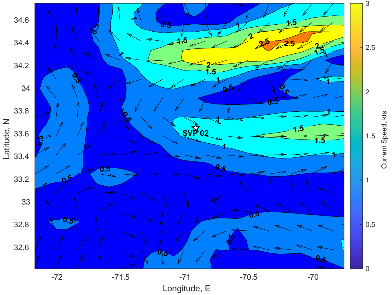
Surface Currents for SVP 02 at 14-Jul-2024 00:00:00
