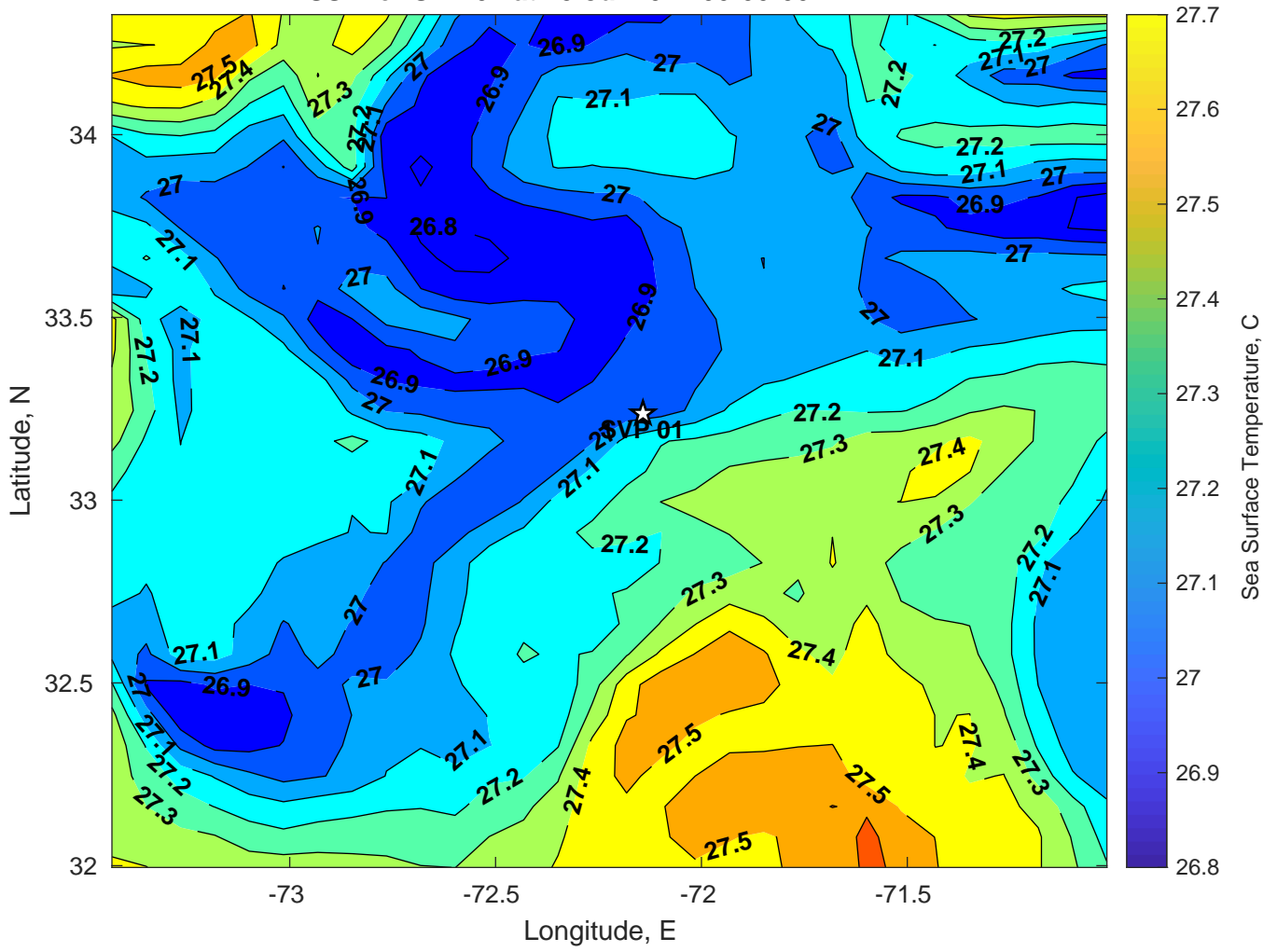
SST for SVP 01 at 15-Jul-2024 00:00:00
