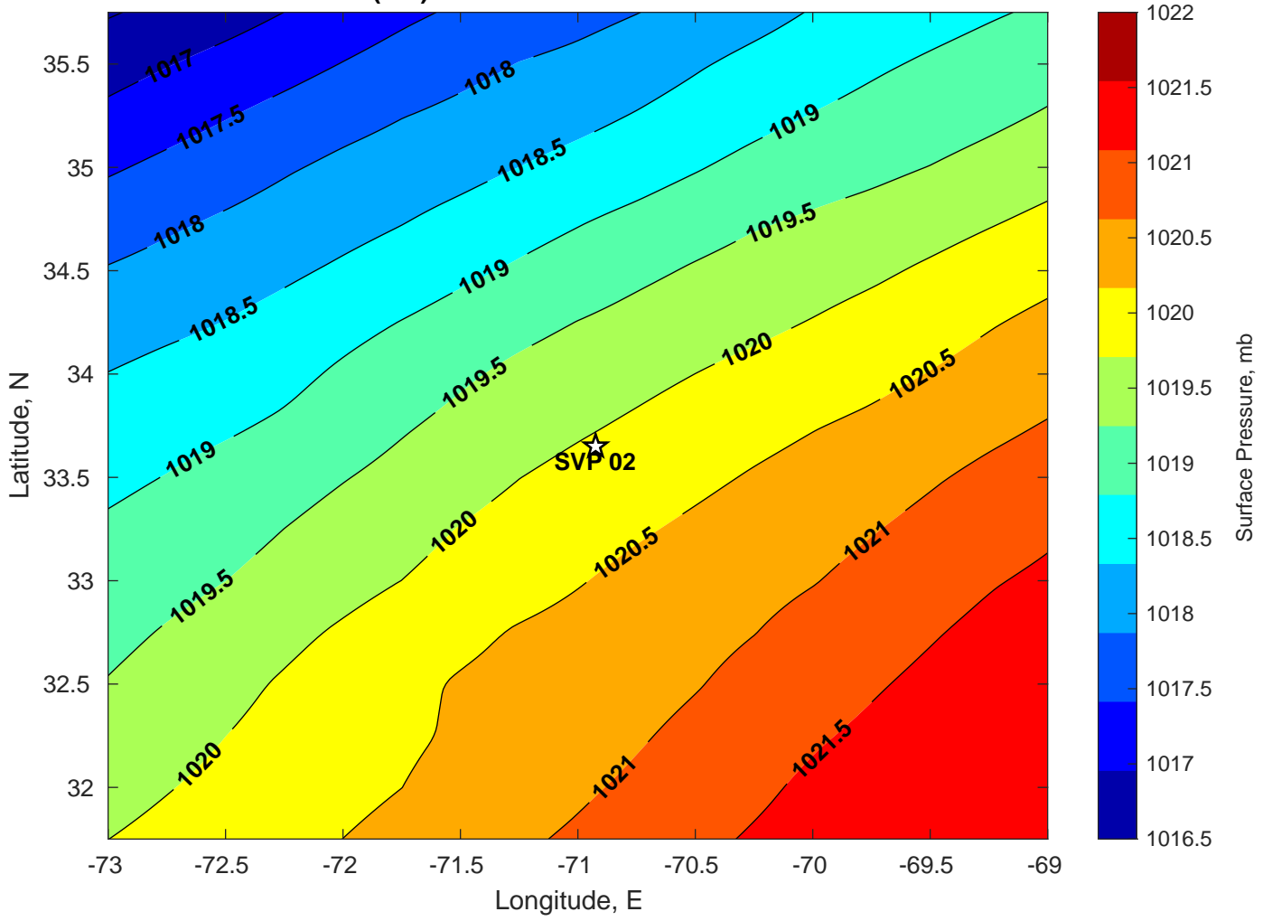
Surface Pressure (mb) for SVP 02 at 17-Jul-2024 00:00:00
