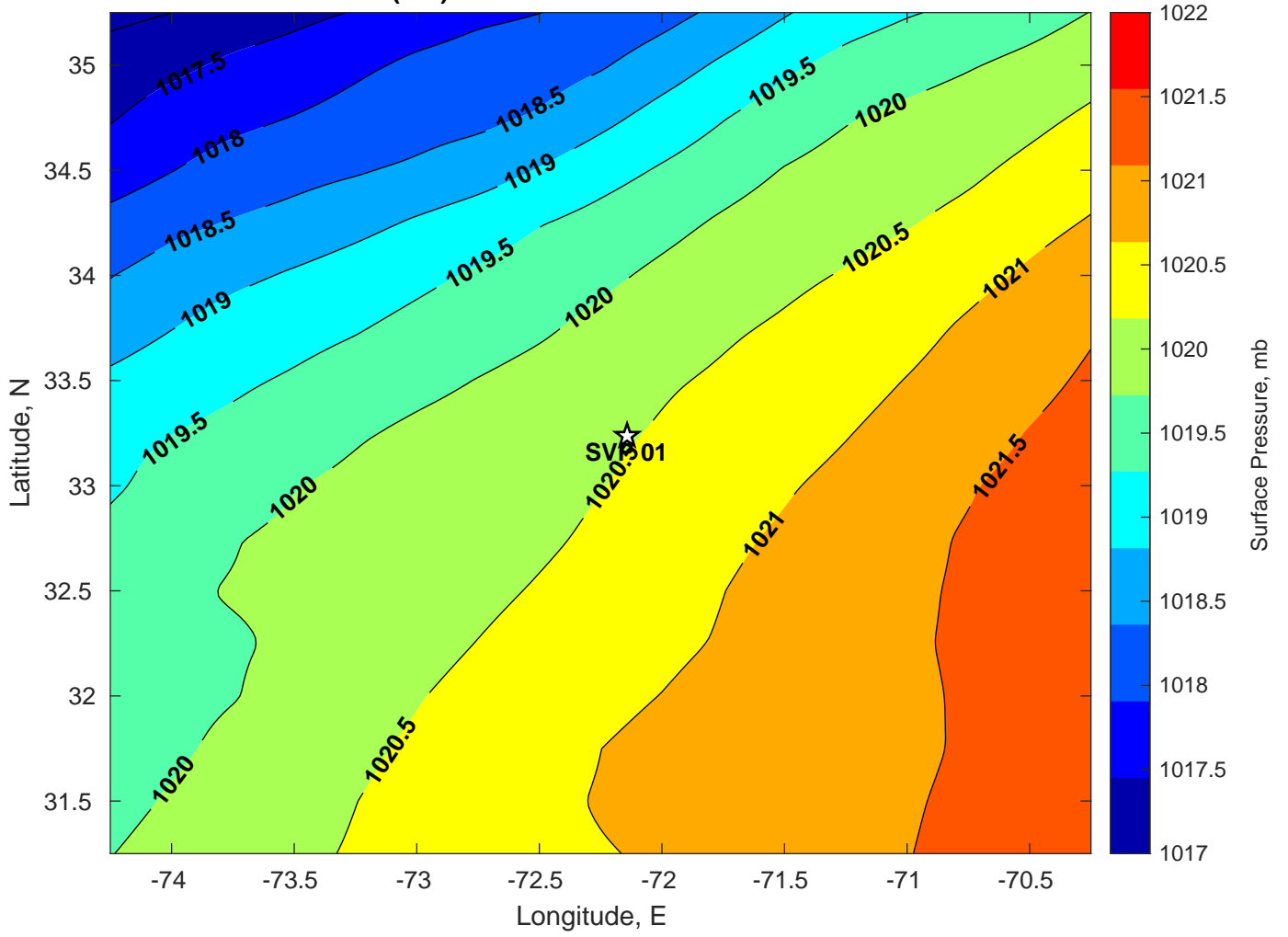
Surface Pressure (mb) for SVP 01 at 18-Jul-2024 00:00:00
