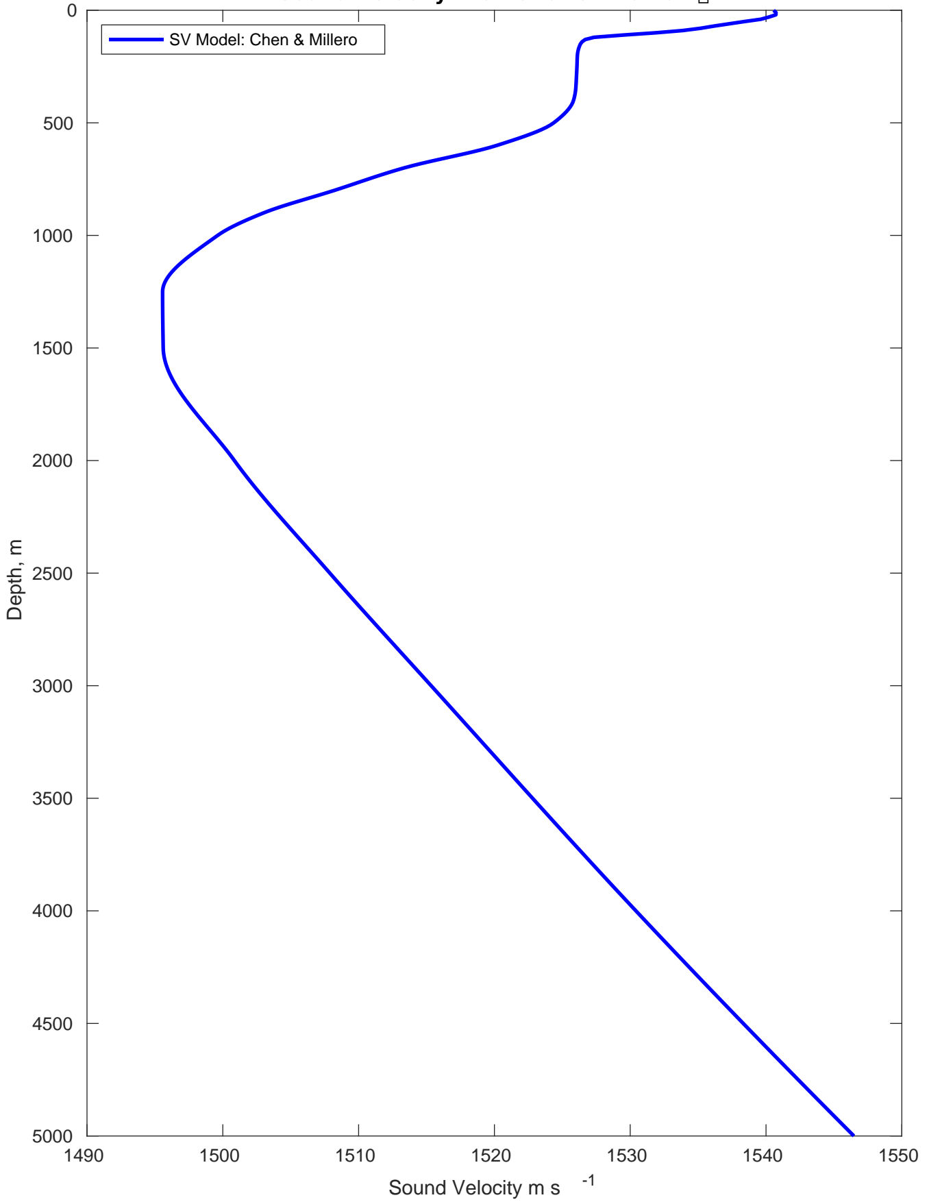
Sound Velocity Profile for SVP 01 on [ ]
