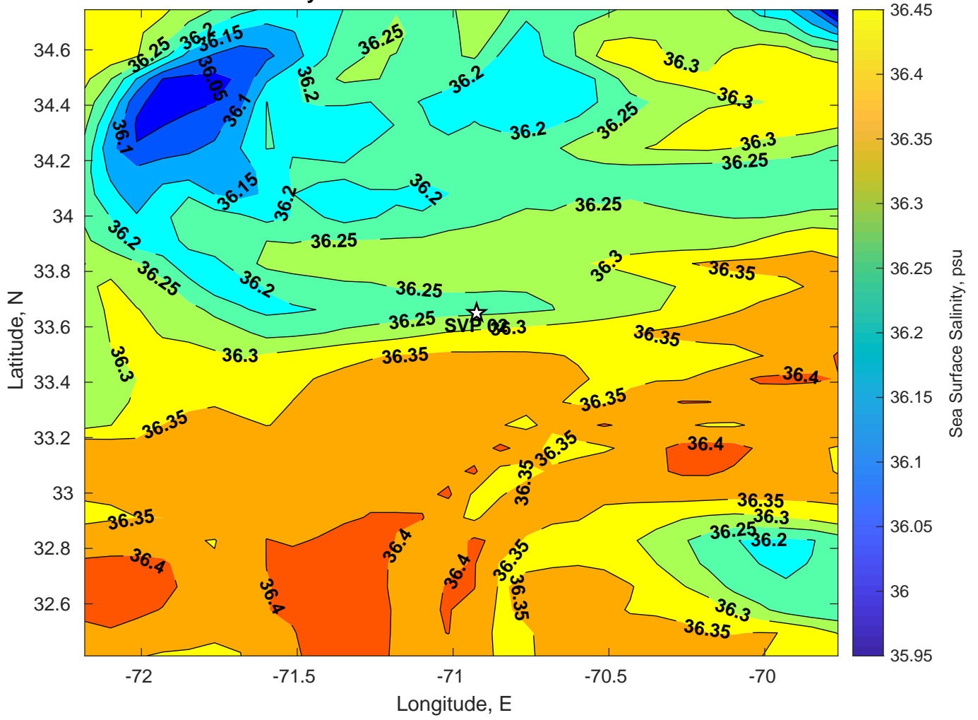
Surface Salinity for SVP 02 at 16-Jul-2024 00:00:00
