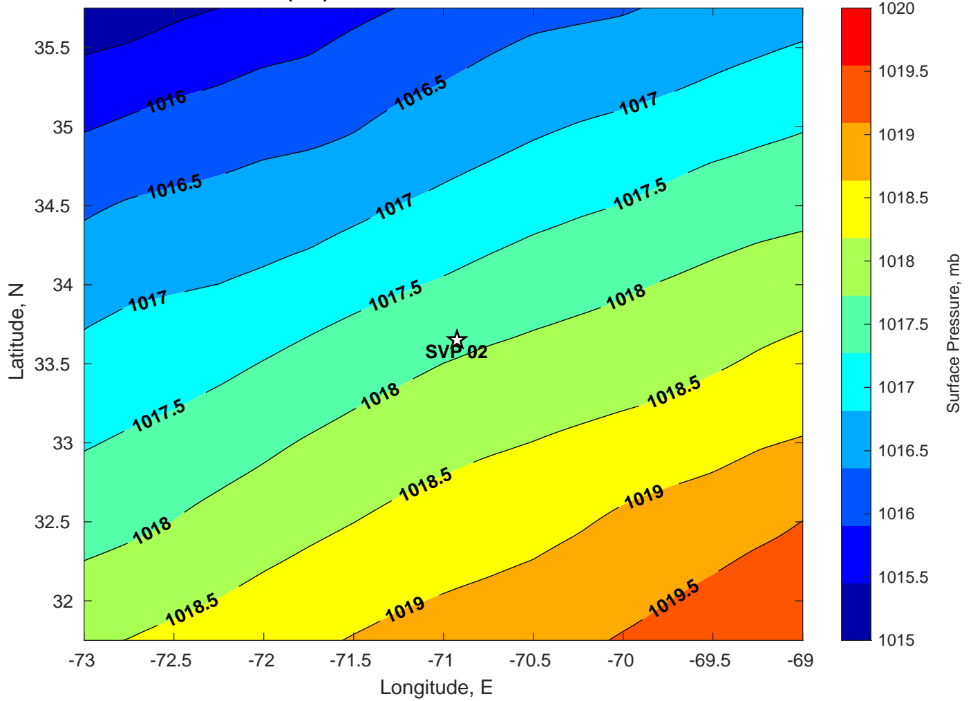
Surface Pressure (mb) for SVP 02 at 16-Jul-2024 00:00:00
