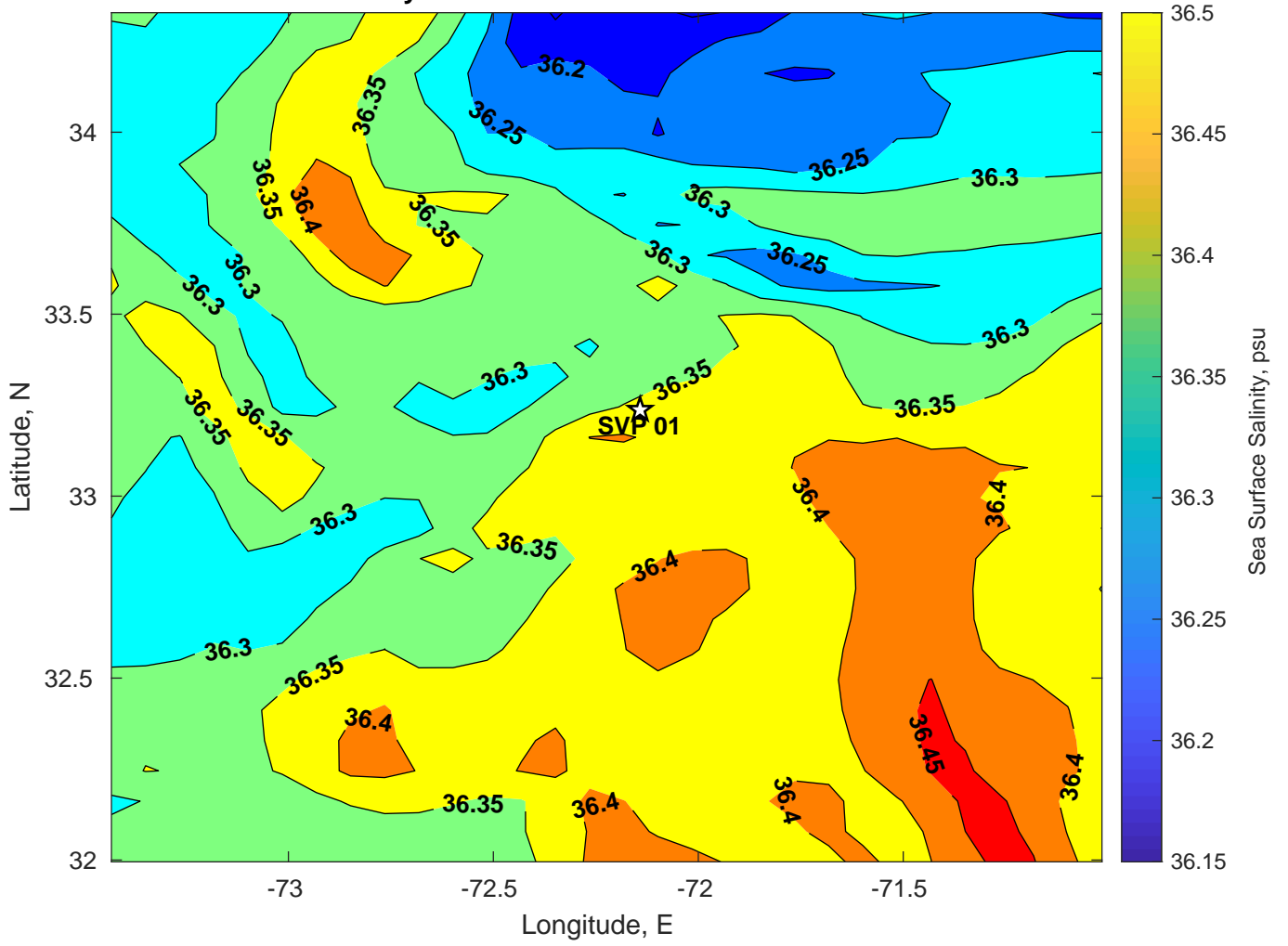
Surface Salinity for SVP 01 at 17-Jul-2024 00:00:00
