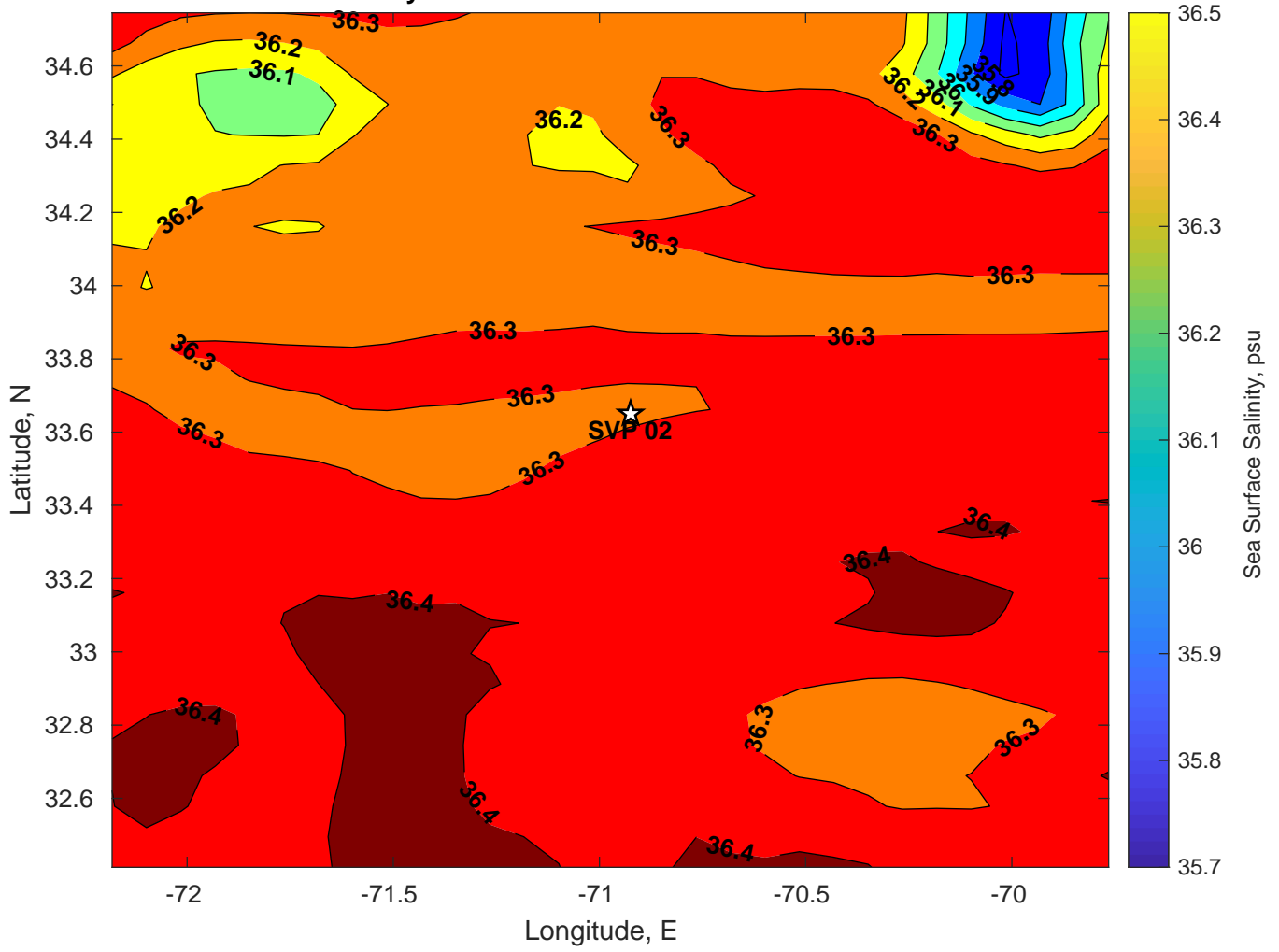
Surface Salinity for SVP 02 at 17-Jul-2024 00:00:00
