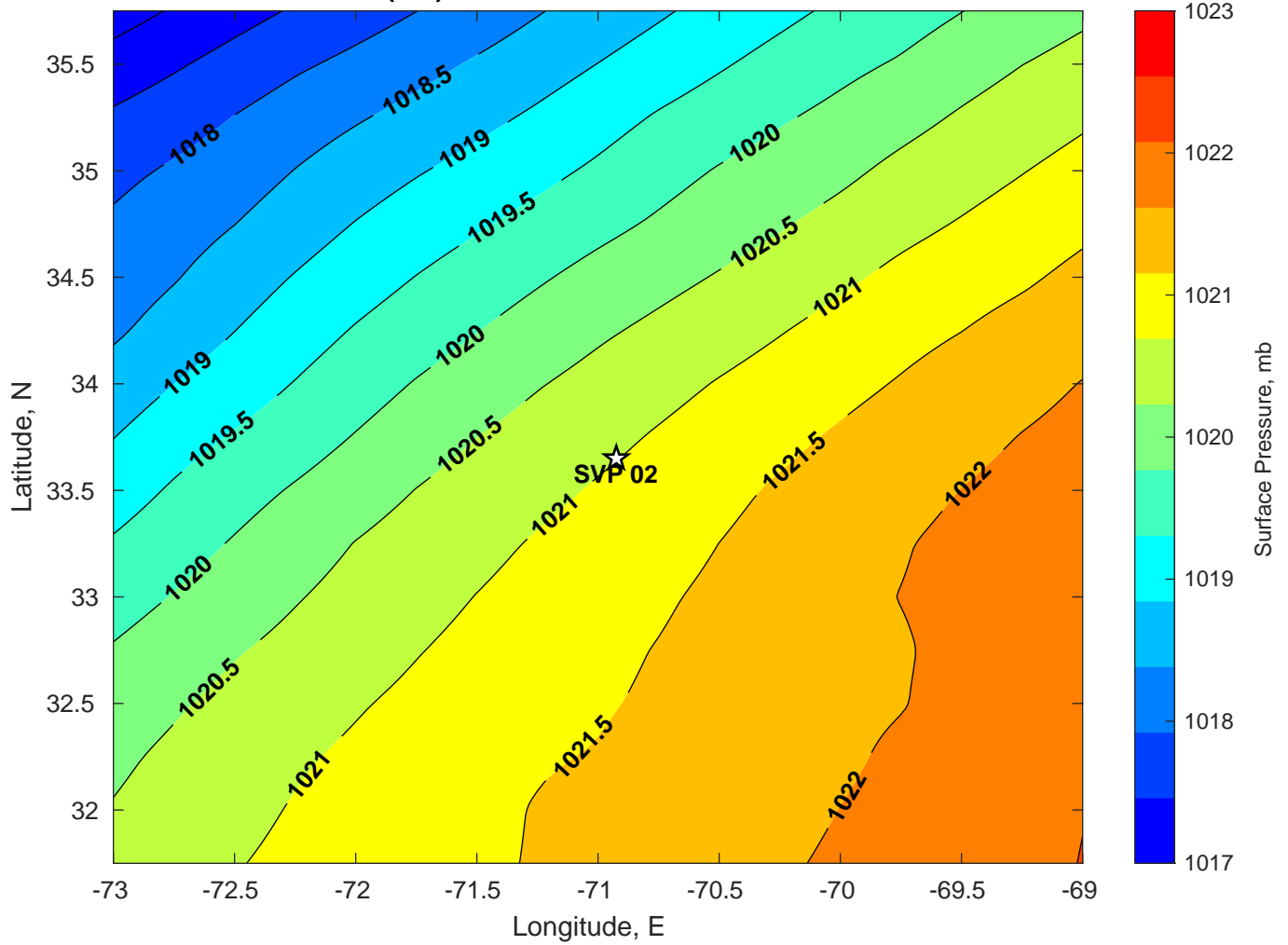
Surface Pressure (mb) for SVP 02 at 18-Jul-2024 00:00:00
