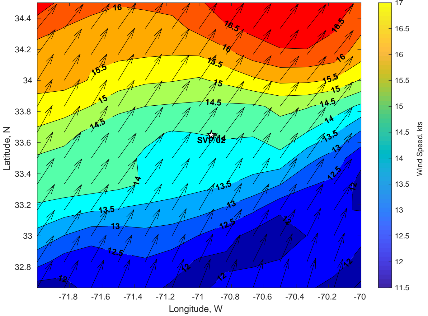
Winds (kts) for SVP 02 at 17-Jul-2024 06:00:00
