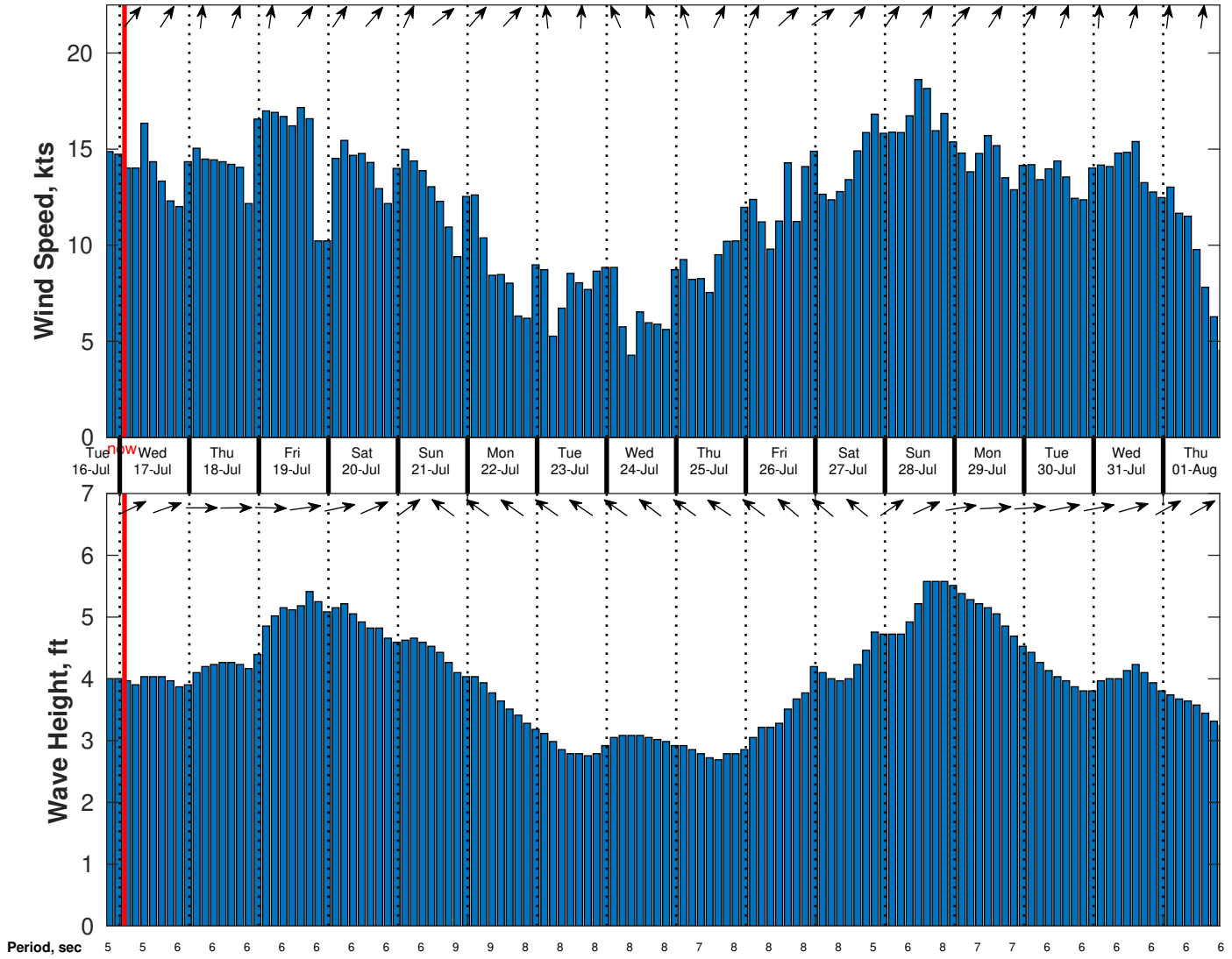
Wind & Wave Forecast for SVP 02 from 16-Jul-2024 19:00:00 to 01-Aug-2024 19:00:00
