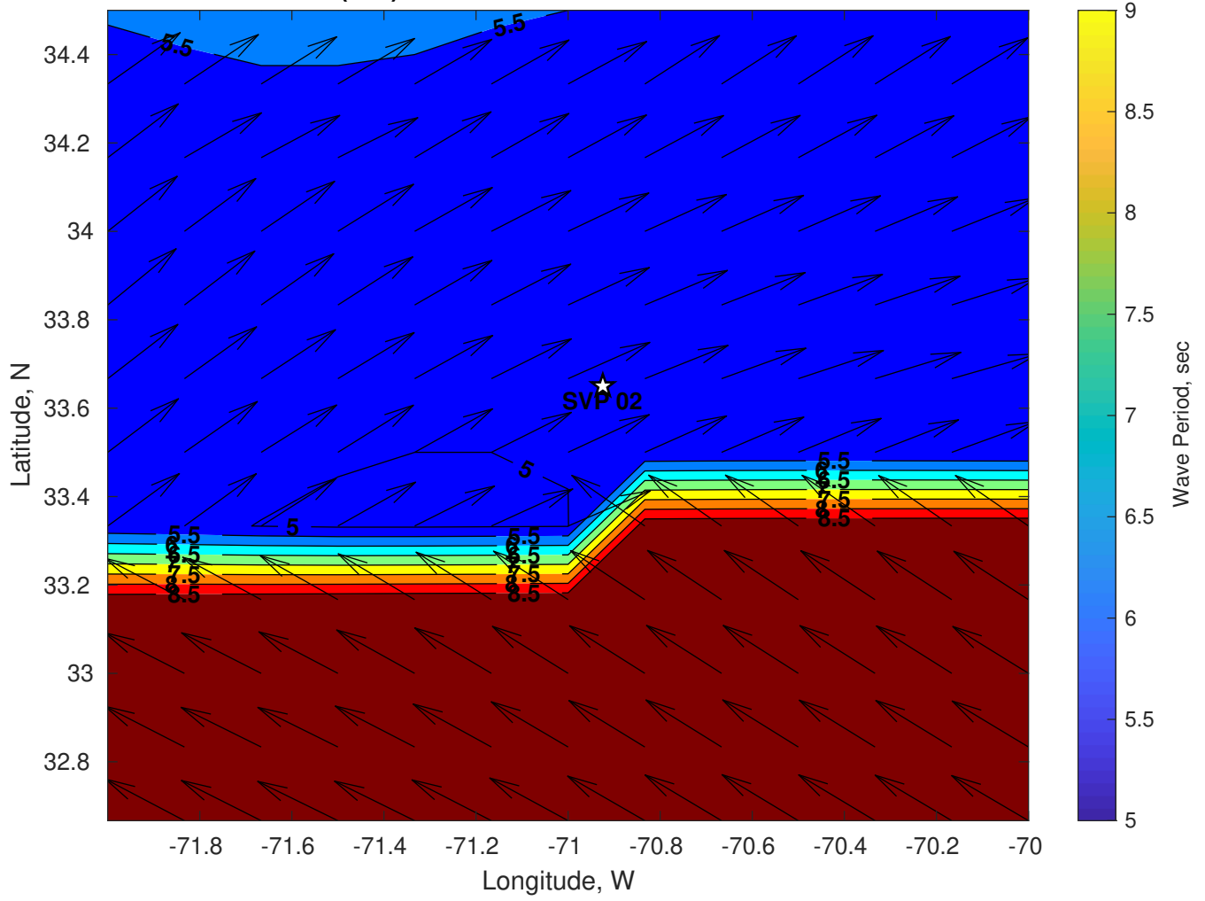
Wave Period (sec) for SVP 02 at 17-Jul-2024 06:00:00
