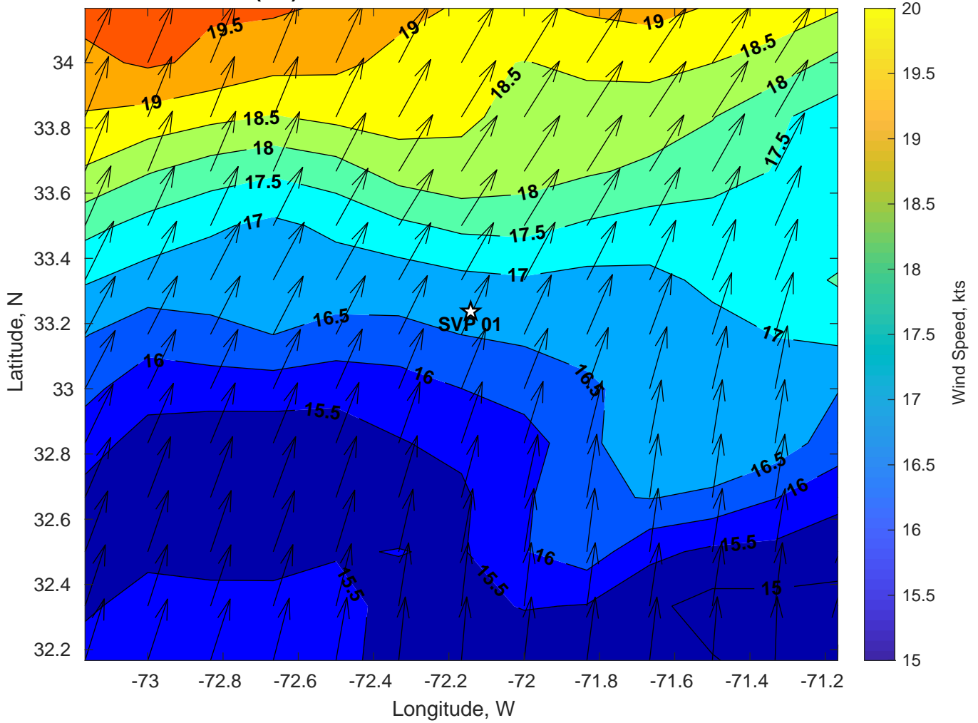
Winds (kts) for SVP 01 at 18-Jul-2024 06:00:00
