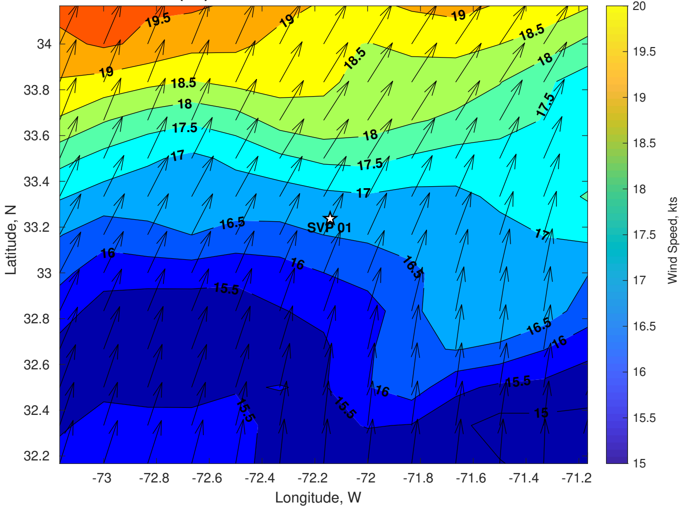
Winds (kts) for SVP 01 at 18-Jul-2024 06:00:00
