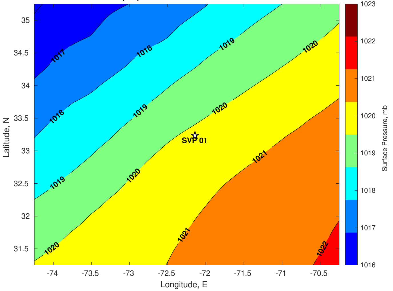
Surface Pressure (mb) for SVP 01 at 18-Jul-2024 00:00:00
