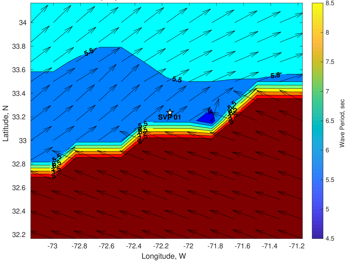
Wave Period (sec) for SVP 01 at 18-Jul-2024 06:00:00
