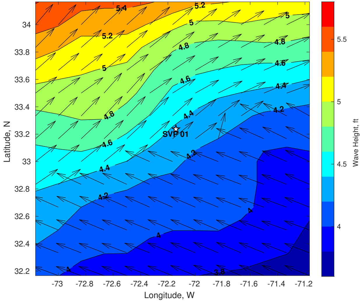
Wave Height (ft) for SVP 01 at 18-Jul-2024 06:00:00
