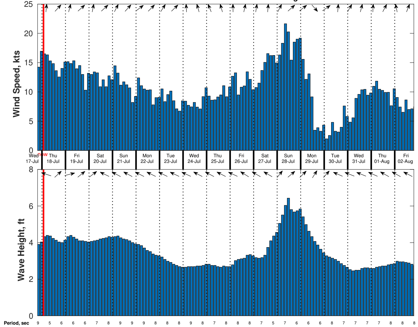
Wind & Wave Forecast for SVP 01 from 17-Jul-2024 19:00:00 to 02-Aug-2024 19:00:00
