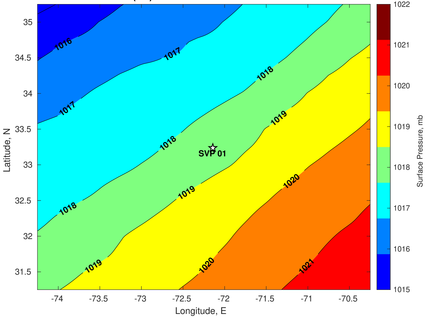
Surface Pressure (mb) for SVP 01 at 19-Jul-2024 00:00:00
