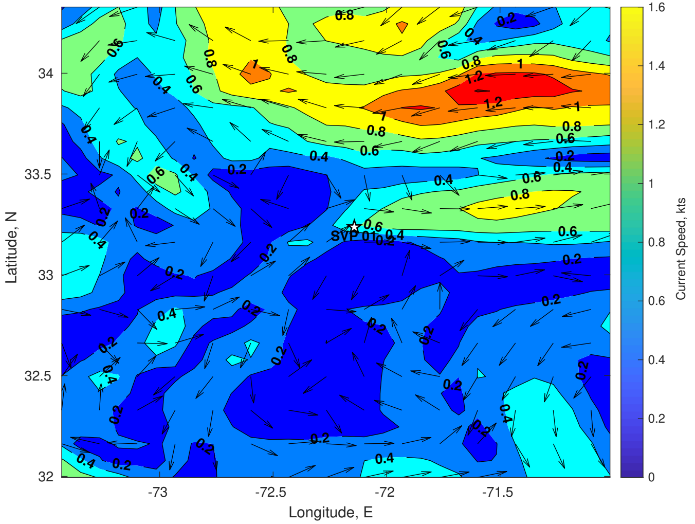
Surface Currents for SVP 01 at 18-Jul-2024 00:00:00
