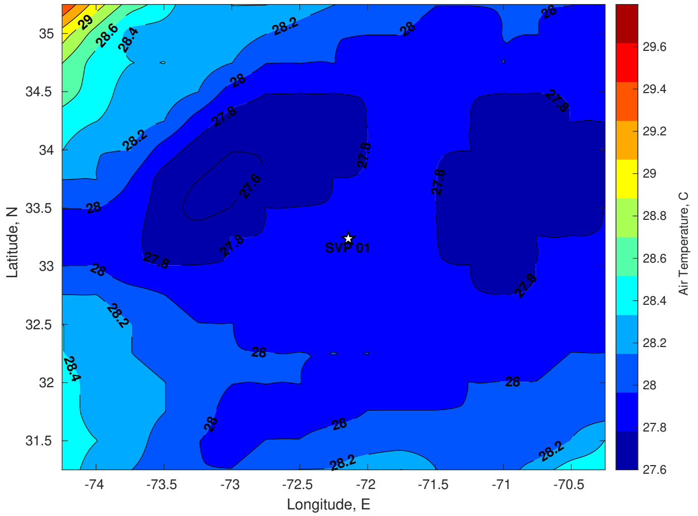
Air Temperature (C) for SVP 01 at 18-Jul-2024
