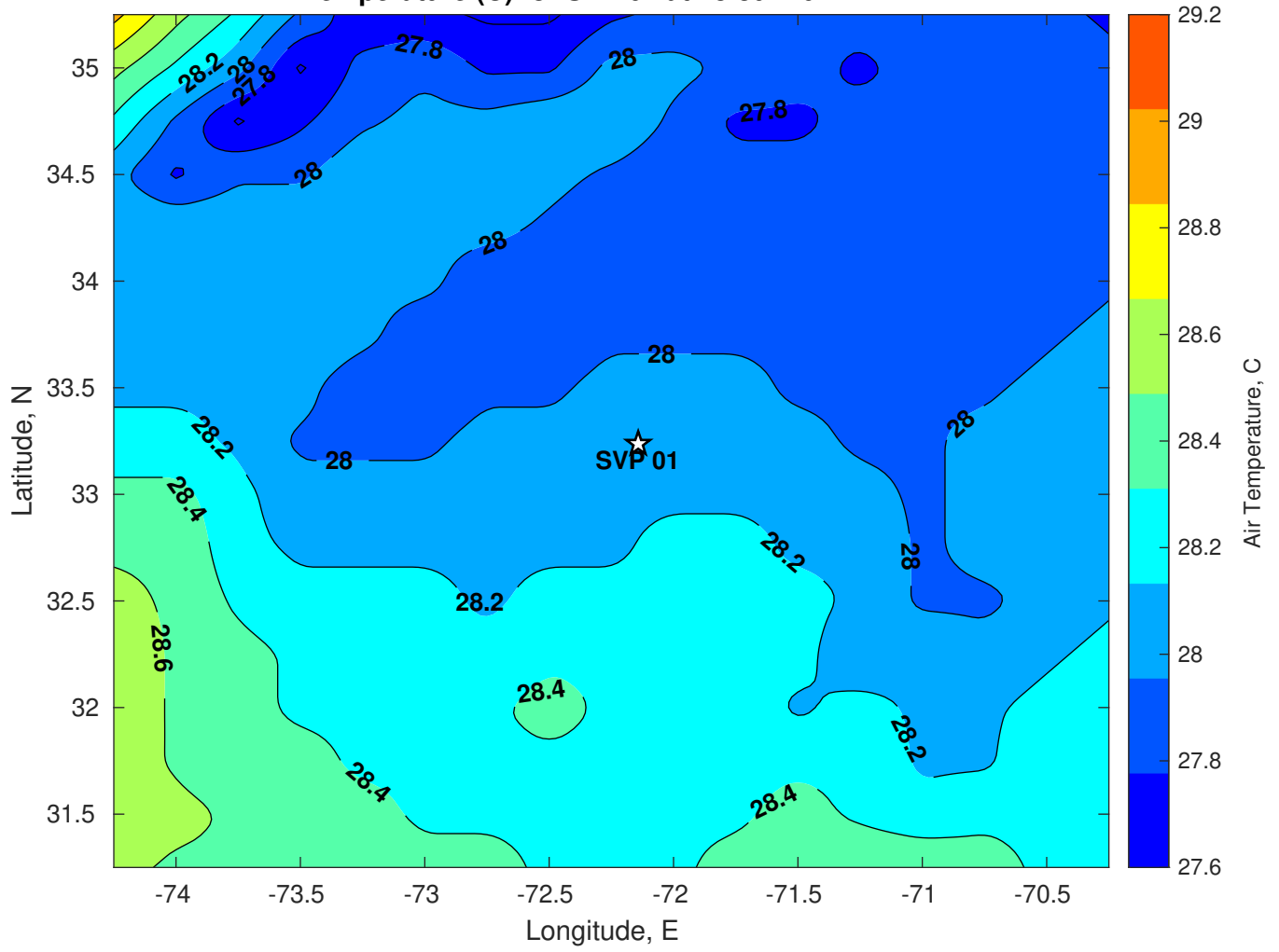
Air Temperature (C) for SVP 01 at 18-Jul-2024
