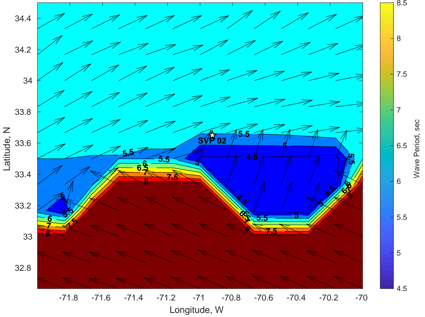
Wave Period (sec) for SVP 02 at 18-Jul-2024 06:00:00
