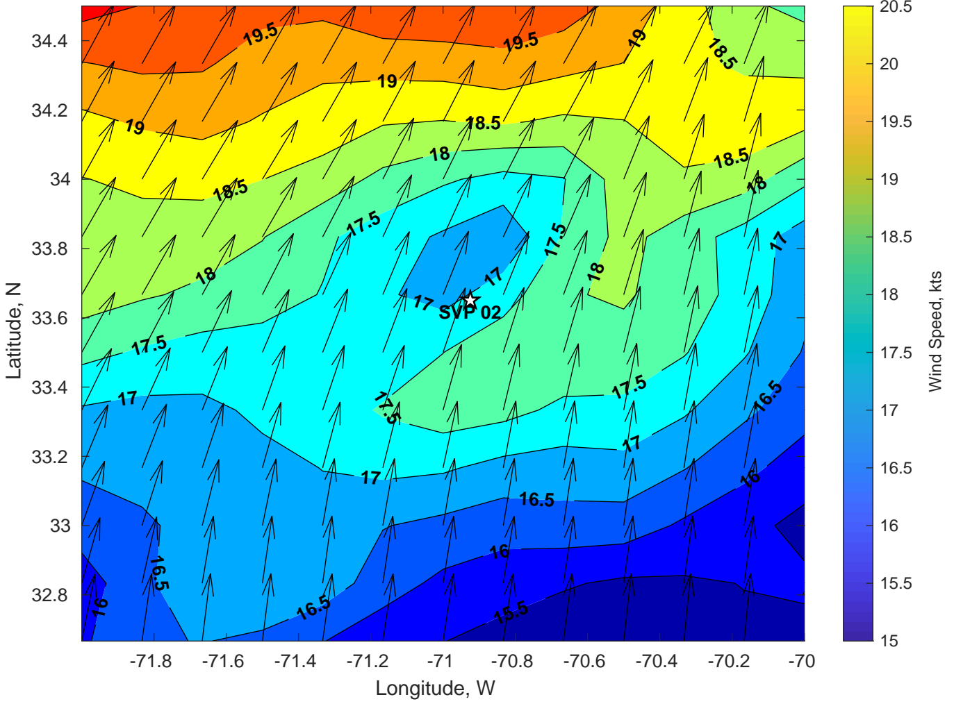
Winds (kts) for SVP 02 at 18-Jul-2024 06:00:00
