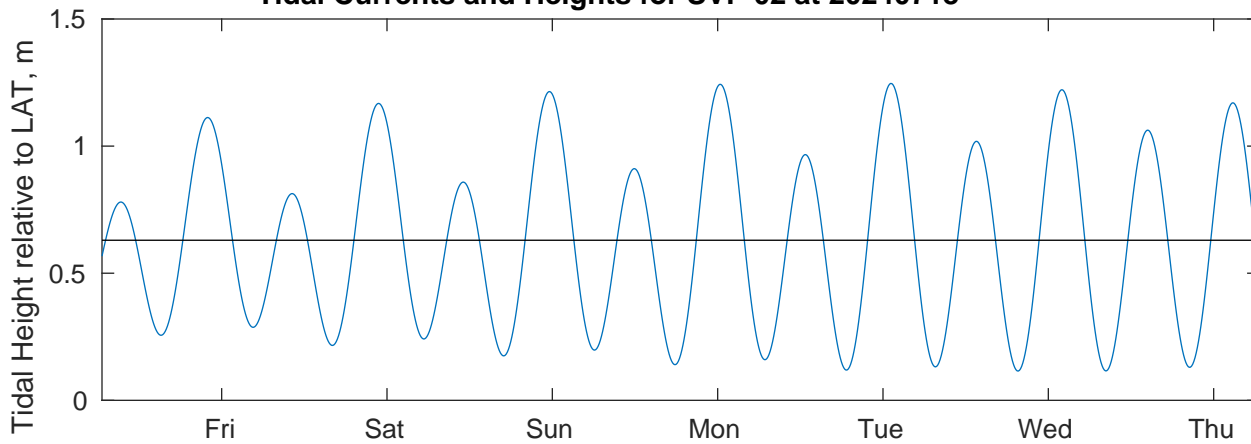
Tidal Currents and Heights for SVP 02 at 20240718
