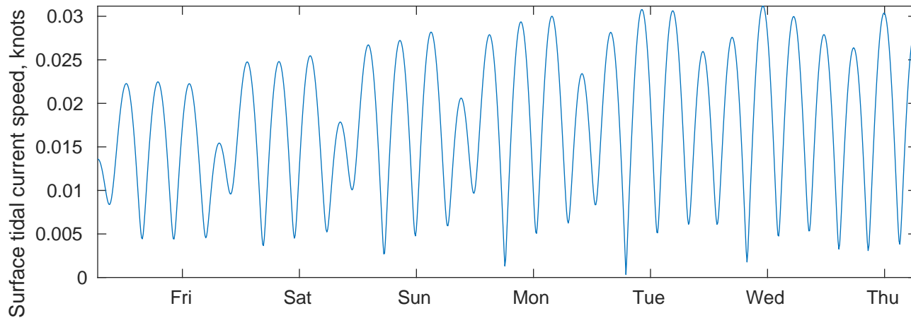
Tidal Currents and Heights for SVP 02 at 20240718
