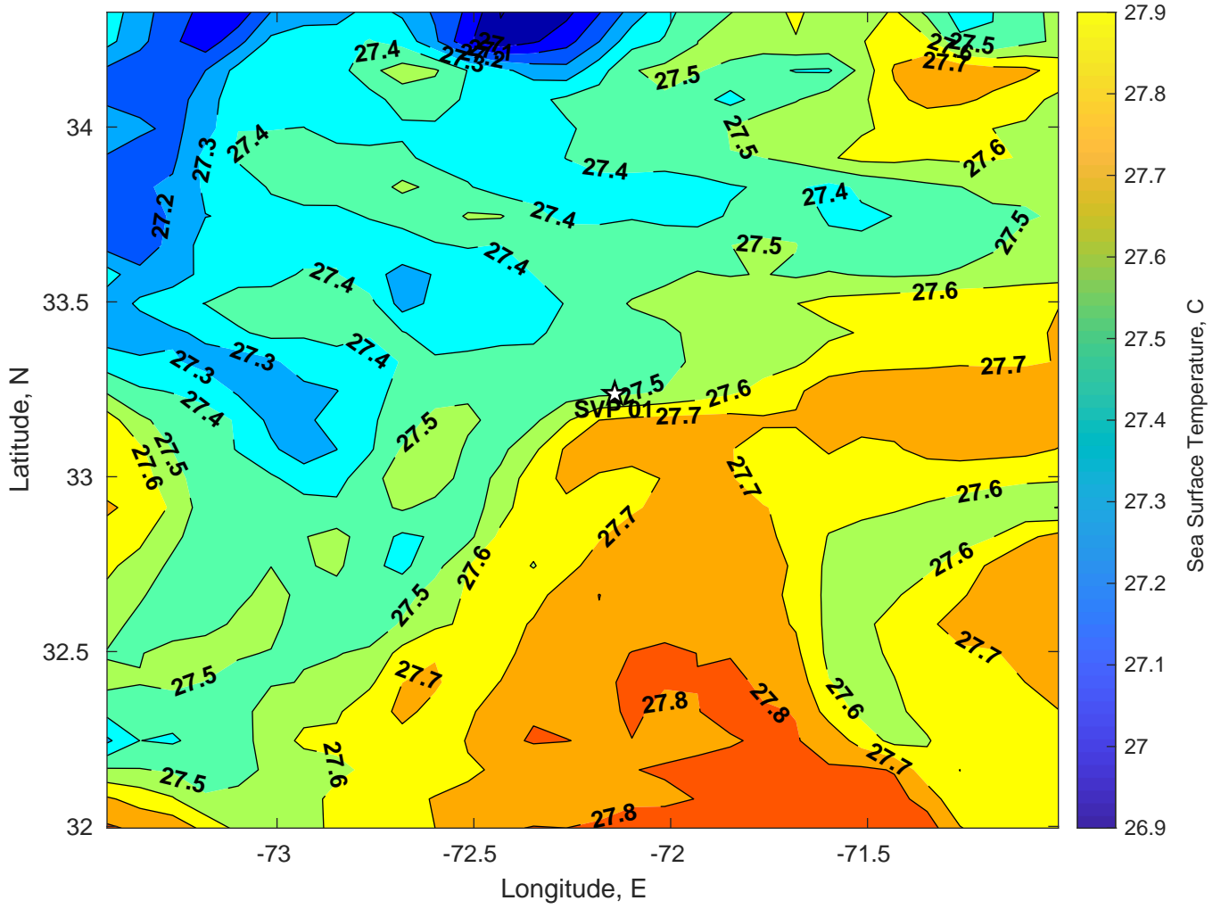
SST for SVP 01 at 19-Jul-2024 00:00:00
