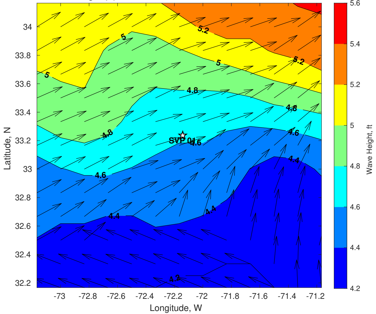
Wave Height (ft) for SVP 01 at 19-Jul-2024 06:00:00
