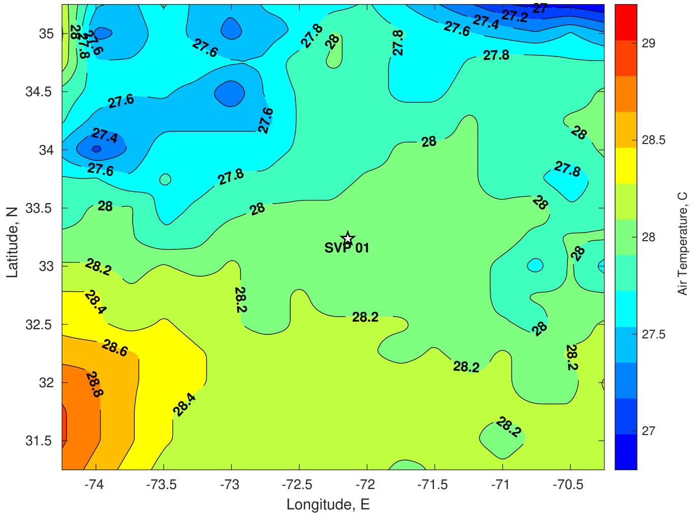
Air Temperature (C) for SVP 01 at 19-Jul-2024
