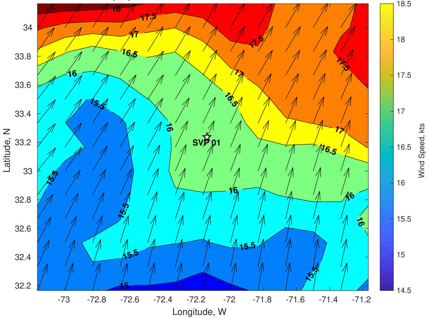
Winds (kts) for SVP 01 at 19-Jul-2024 06:00:00
