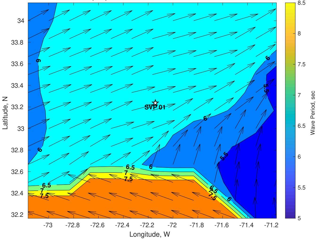
Wave Period (sec) for SVP 01 at 19-Jul-2024 06:00:00
