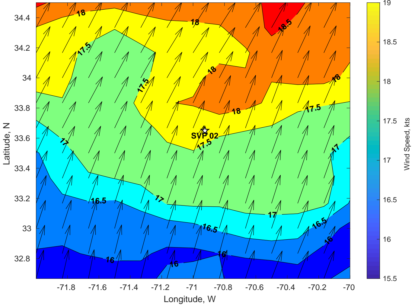
Winds (kts) for SVP 02 at 19-Jul-2024 06:00:00
