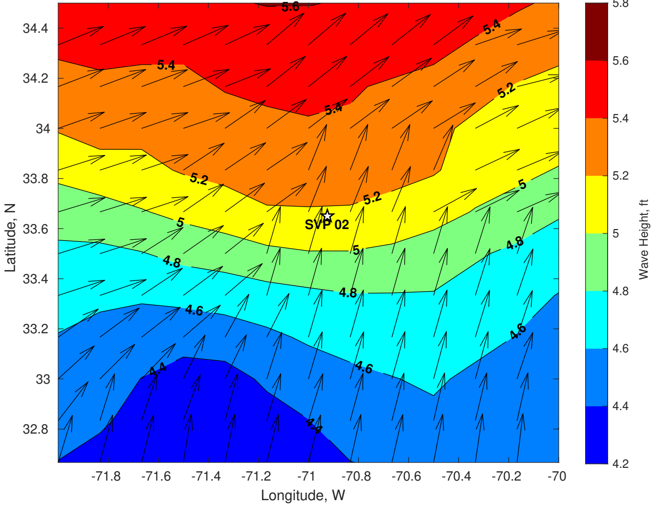
Wave Height (ft) for SVP 02 at 19-Jul-2024 06:00:00
