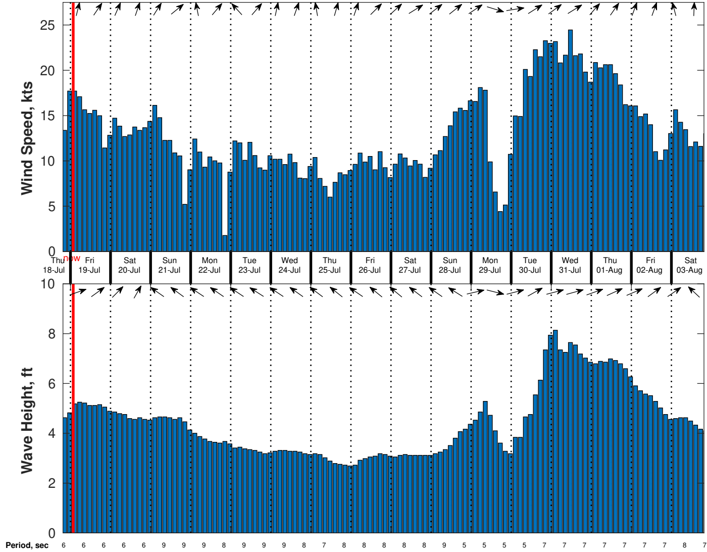
Wind & Wave Forecast for SVP 02 from 18-Jul-2024 19:00:00 to 03-Aug-2024 19:00:00
