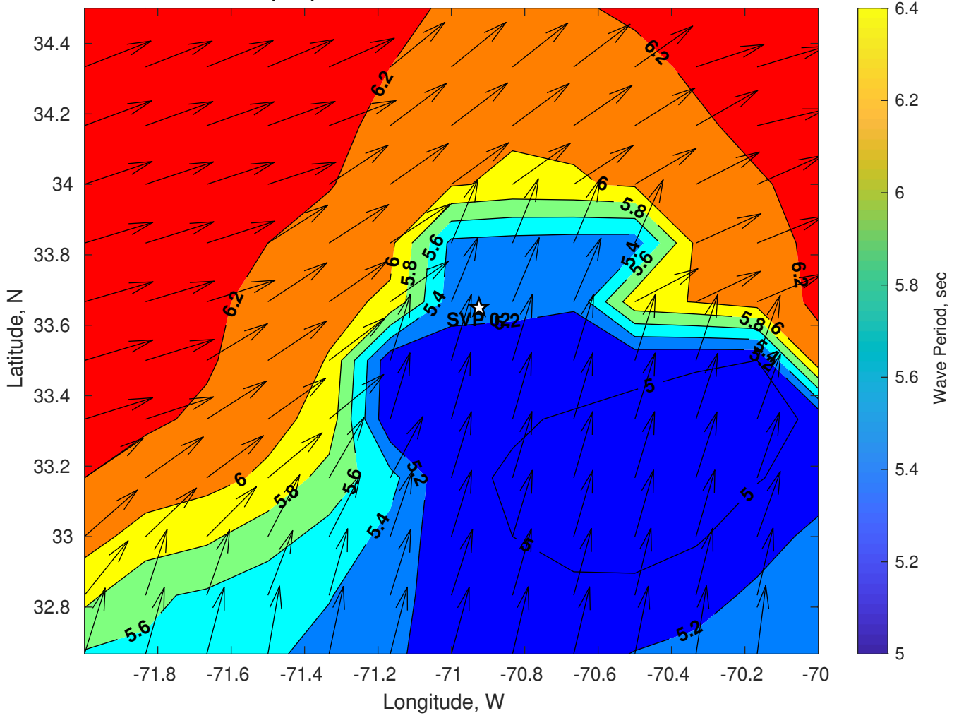
Wave Period (sec) for SVP 02 at 19-Jul-2024 06:00:00
