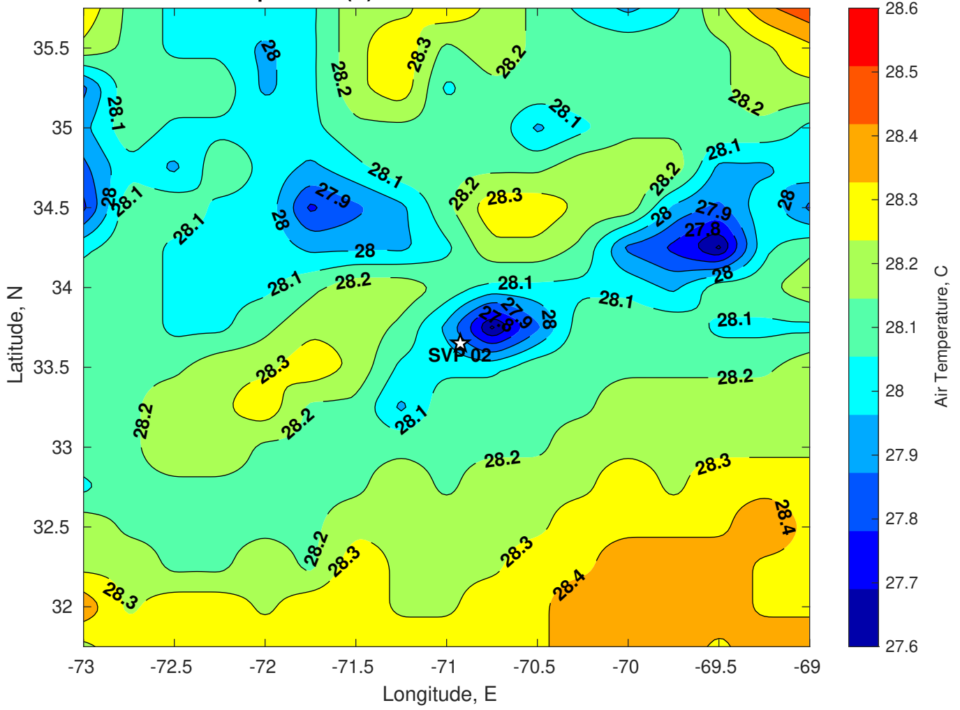
Air Temperature (C) for SVP 02 at 19-Jul-2024
