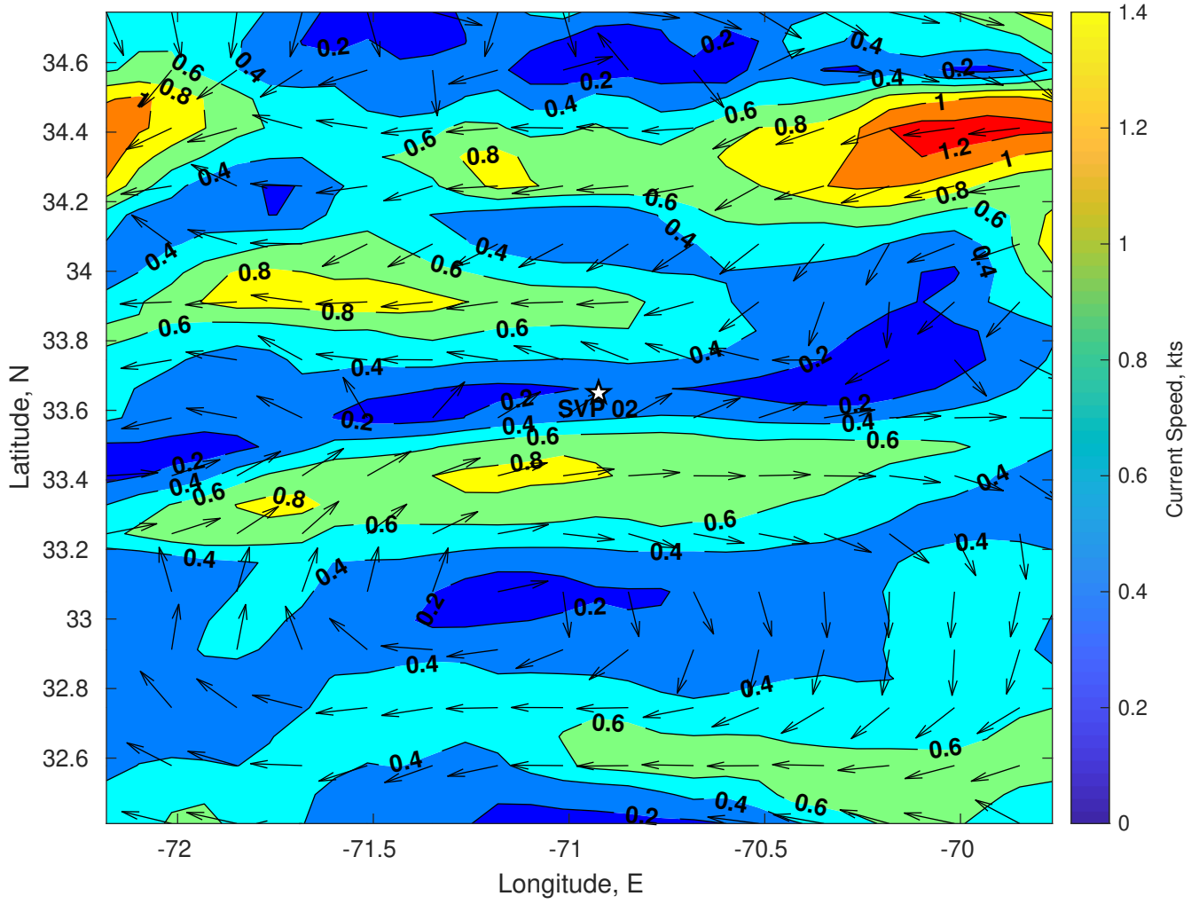
Surface Currents for SVP 02 at 19-Jul-2024 00:00:00
