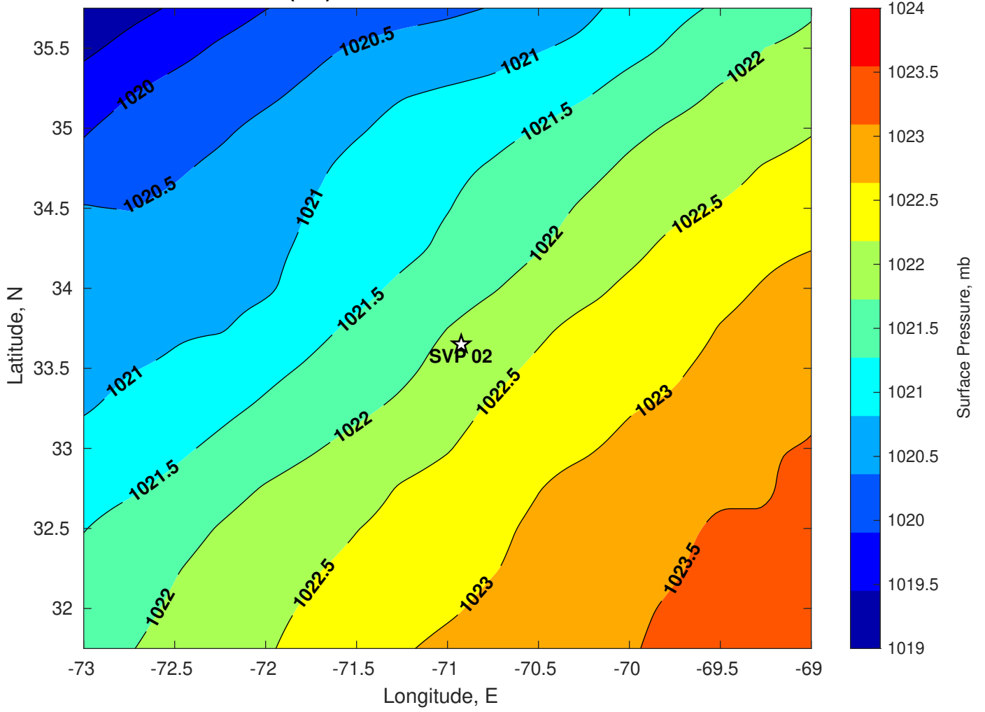
Surface Pressure (mb) for SVP 02 at 20-Jul-2024 00:00:00
