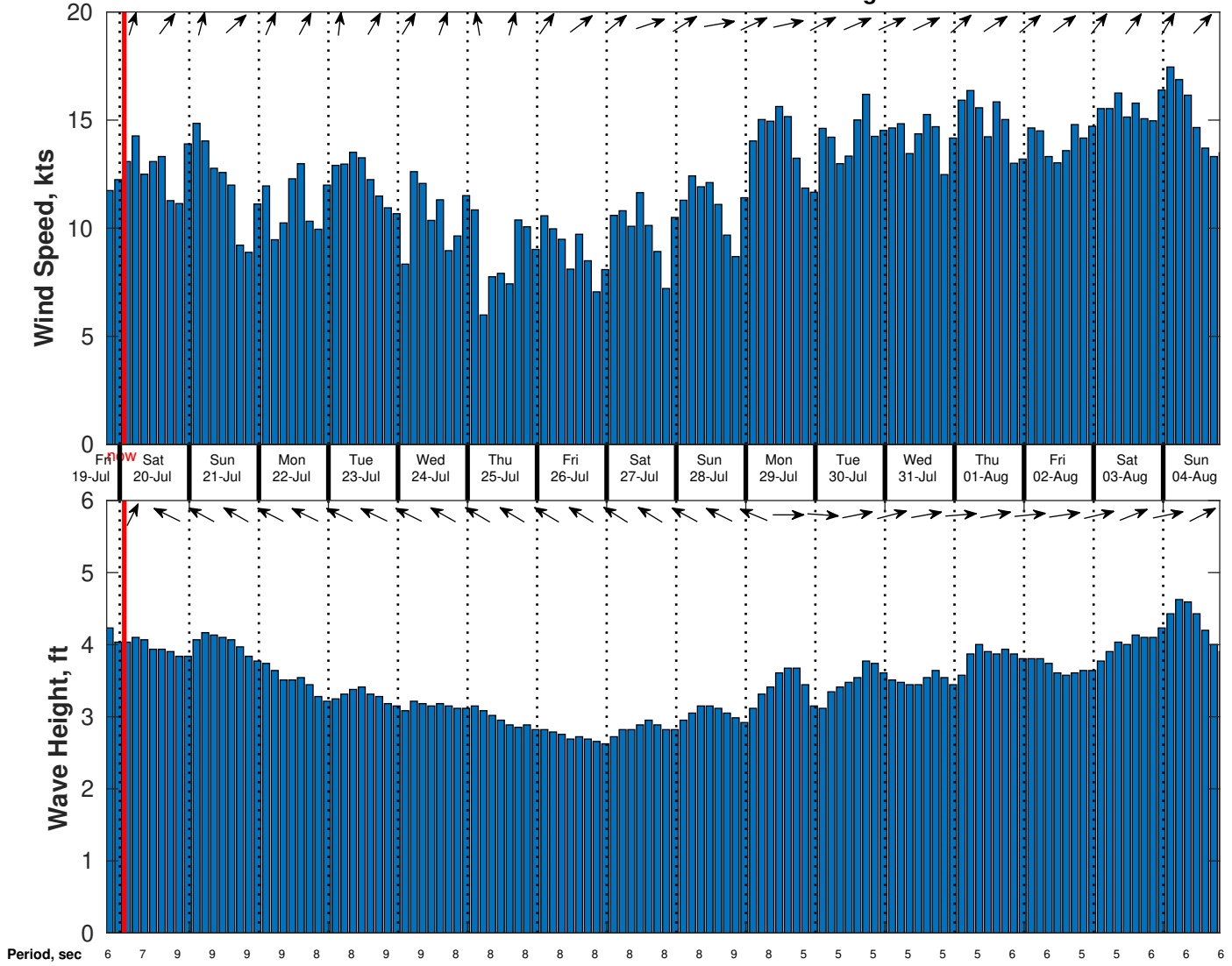
Wind & Wave Forecast for SVP 01 from 19-Jul-2024 19:00:00 to 04-Aug-2024 19:00:00
