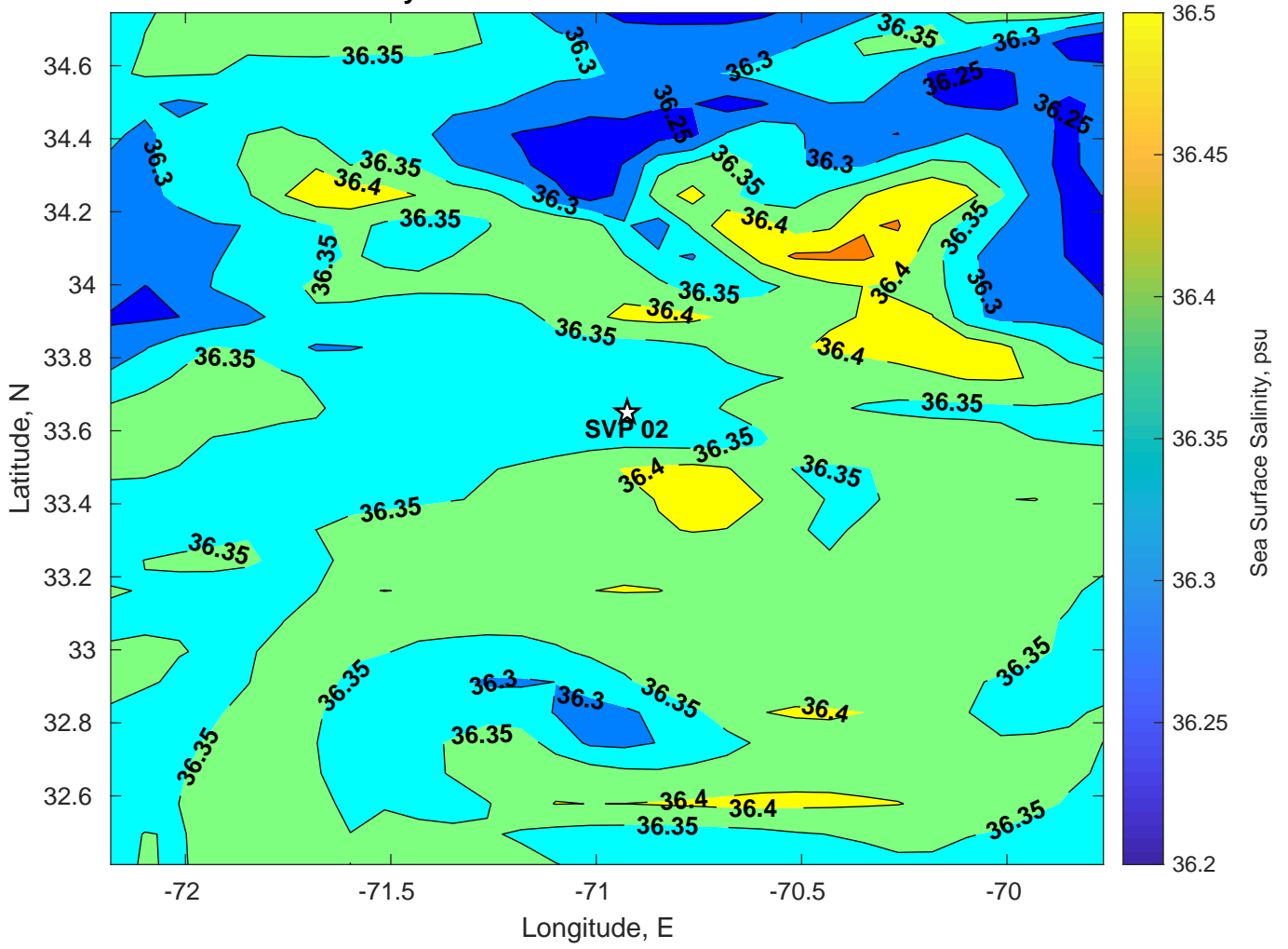
Surface Salinity for SVP 02 at 20-Jul-2024 00:00:00
