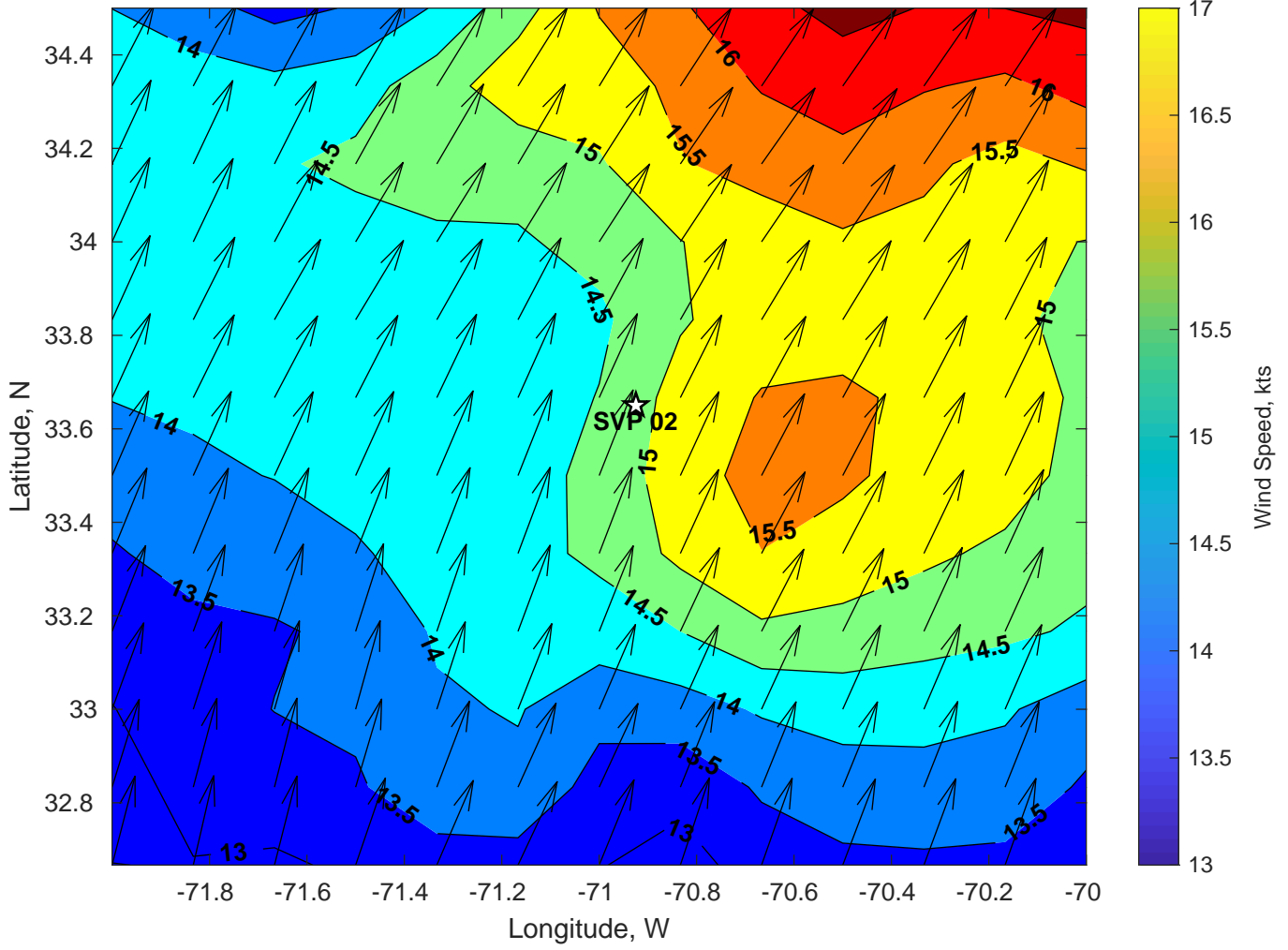
Winds (kts) for SVP 02 at 20-Jul-2024 06:00:00
