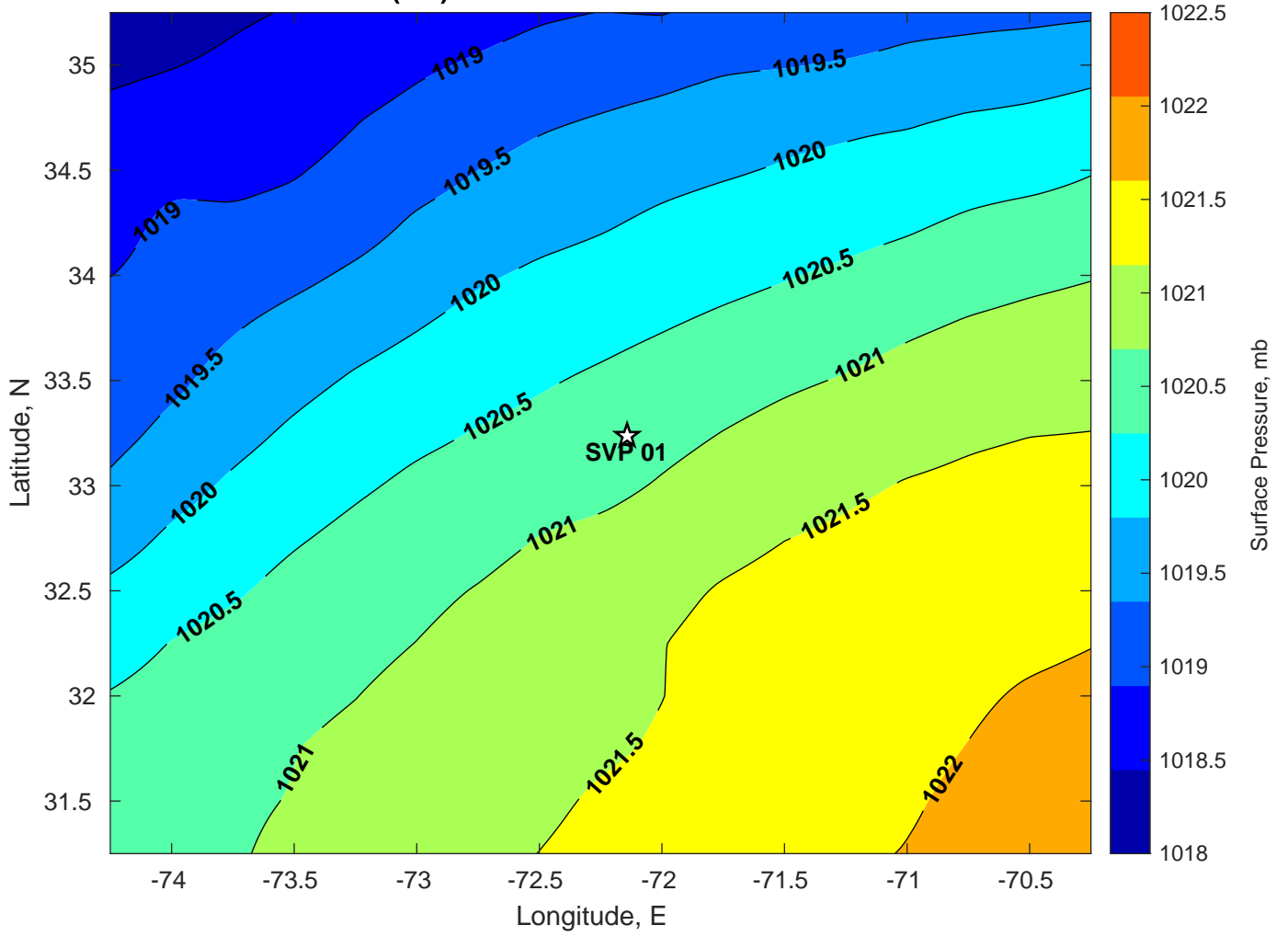
Surface Pressure (mb) for SVP 01 at 22-Jul-2024 00:00:00
