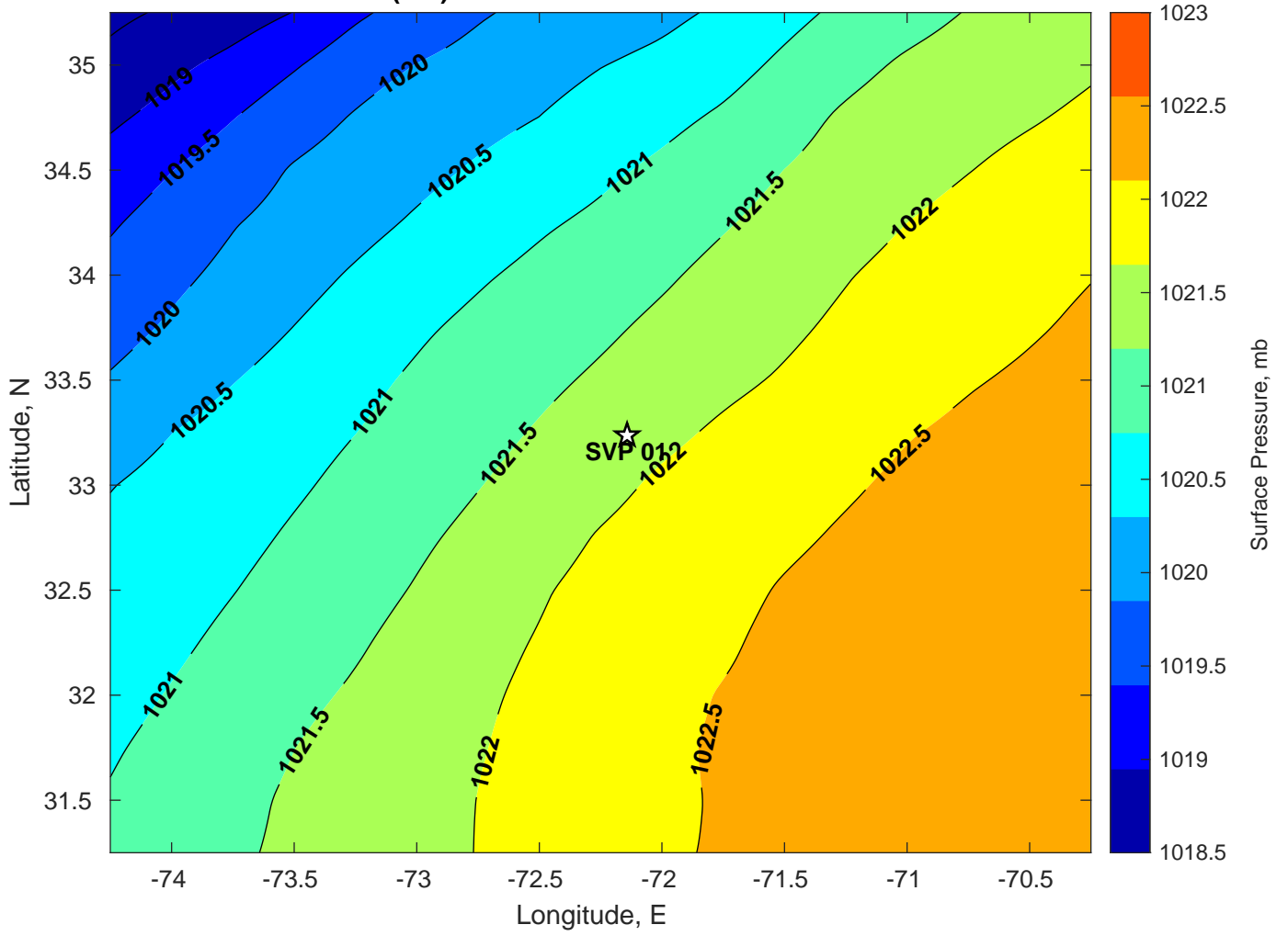
Surface Pressure (mb) for SVP 01 at 23-Jul-2024 00:00:00
