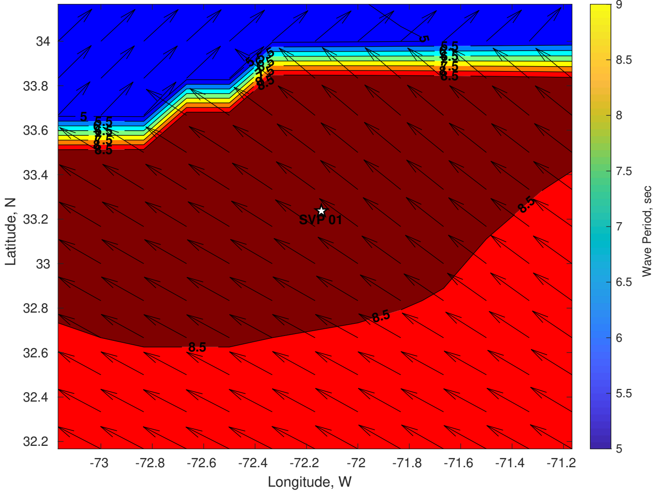
Wave Period (sec) for SVP 01 at 21-Jul-2024 06:00:00
