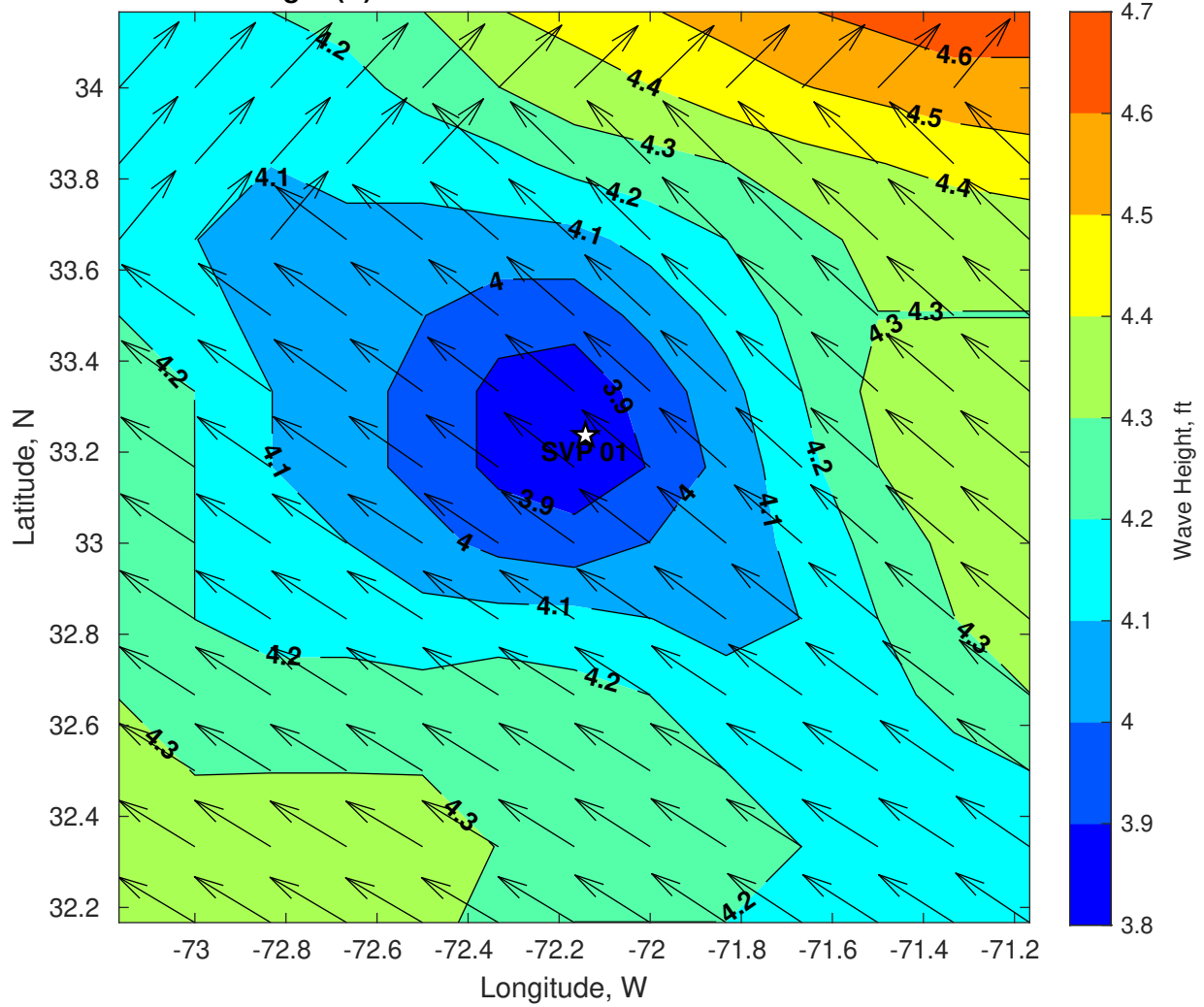
Wave Height (ft) for SVP 01 at 21-Jul-2024 06:00:00
