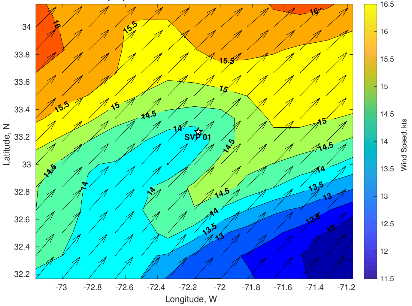
Winds (kts) for SVP 01 at 21-Jul-2024 06:00:00
