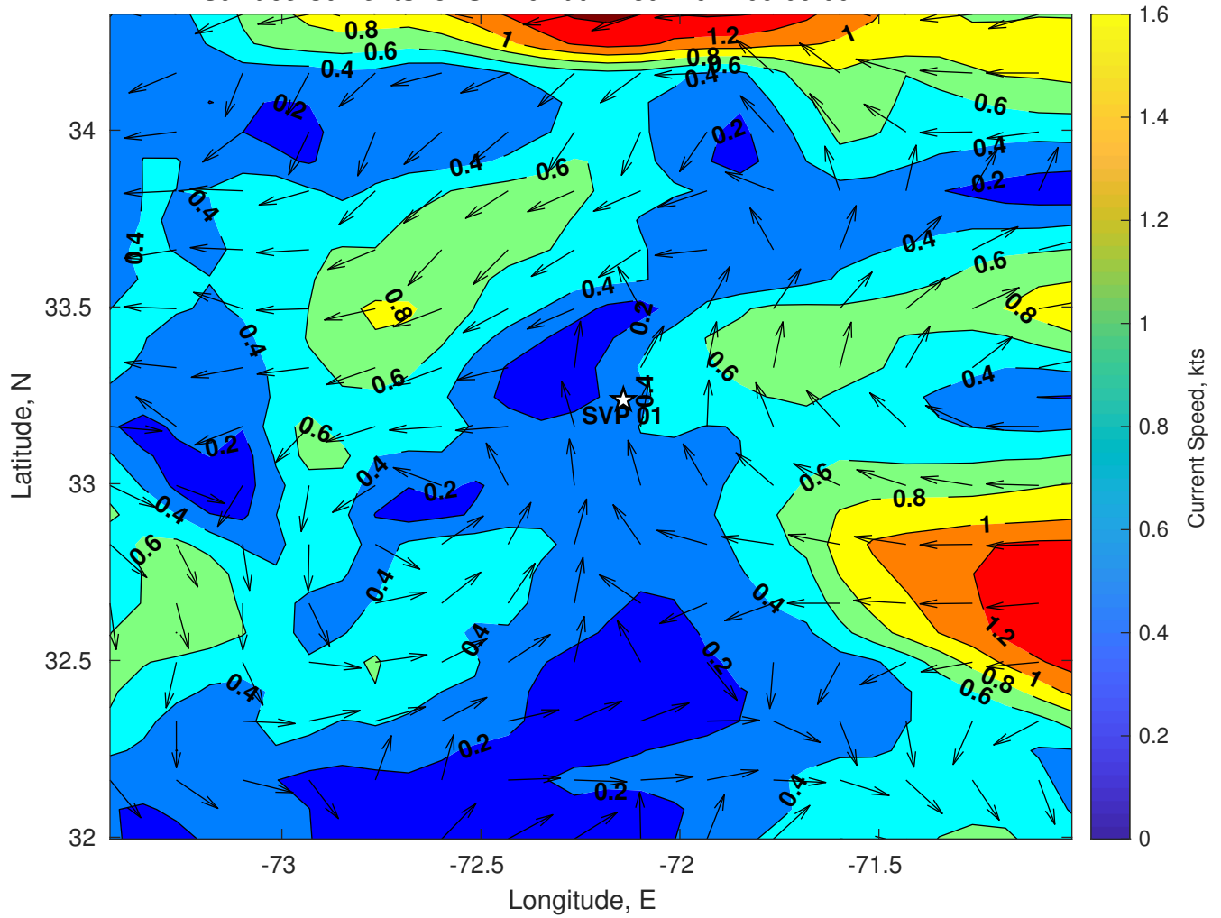
Surface Currents for SVP 01 at 21-Jul-2024 00:00:00
