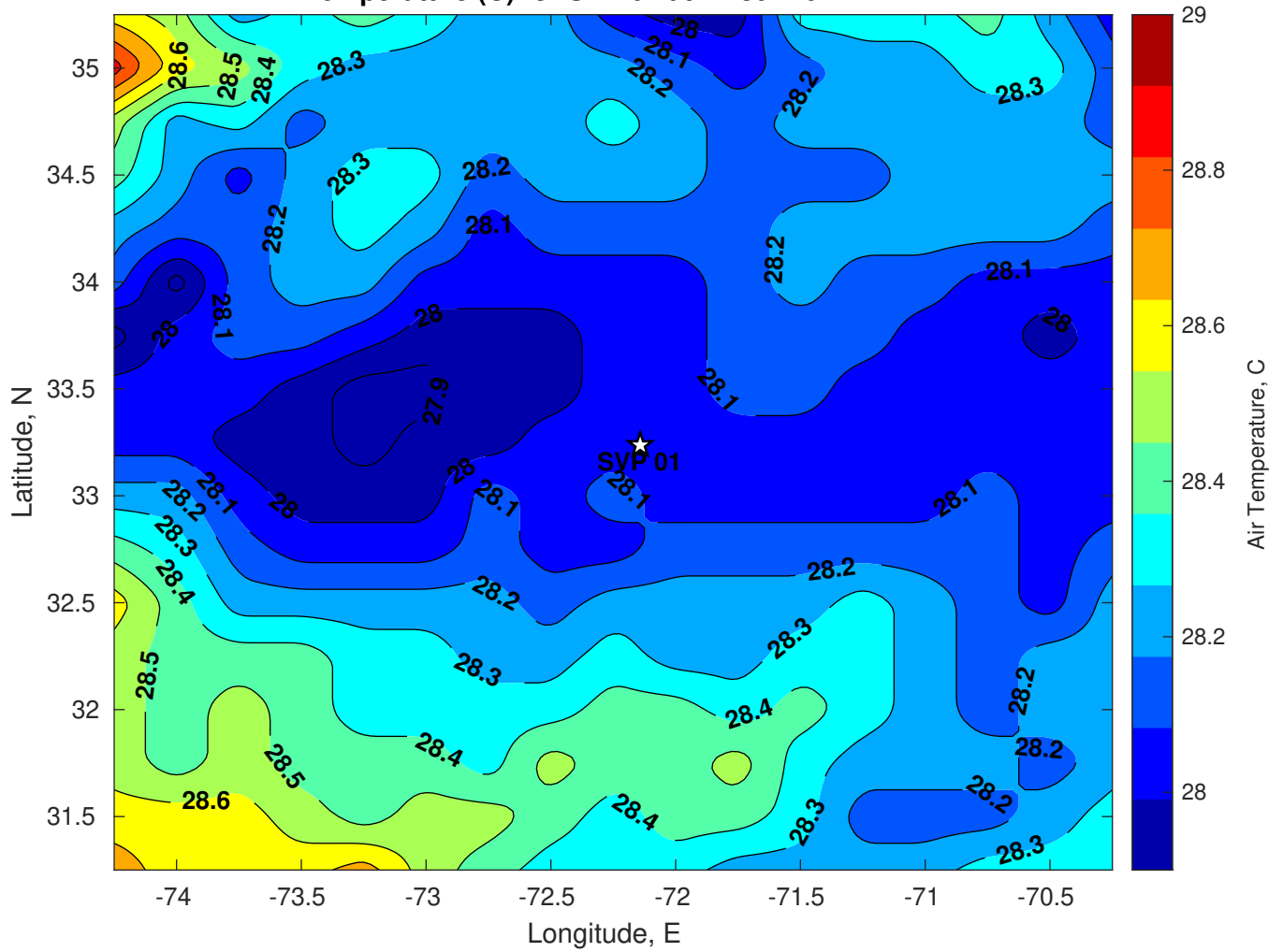
Air Temperature (C) for SVP 01 at 21-Jul-2024
