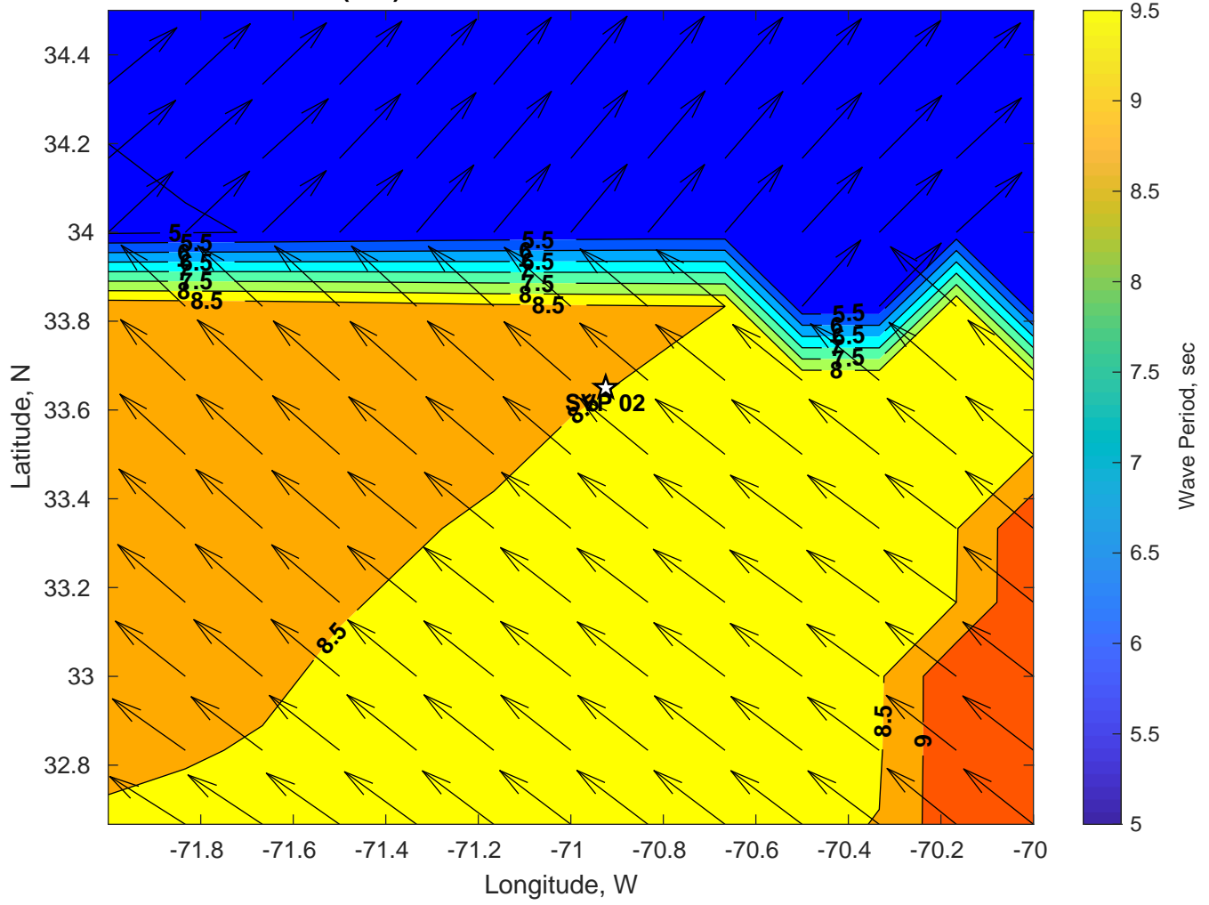
Wave Period (sec) for SVP 02 at 21-Jul-2024 06:00:00
