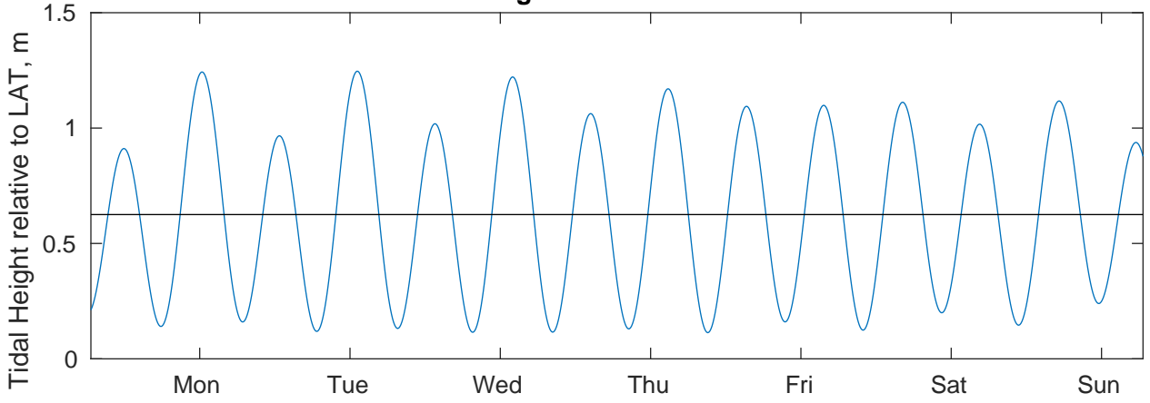
Tidal Currents and Heights for SVP 02 at 20240721
