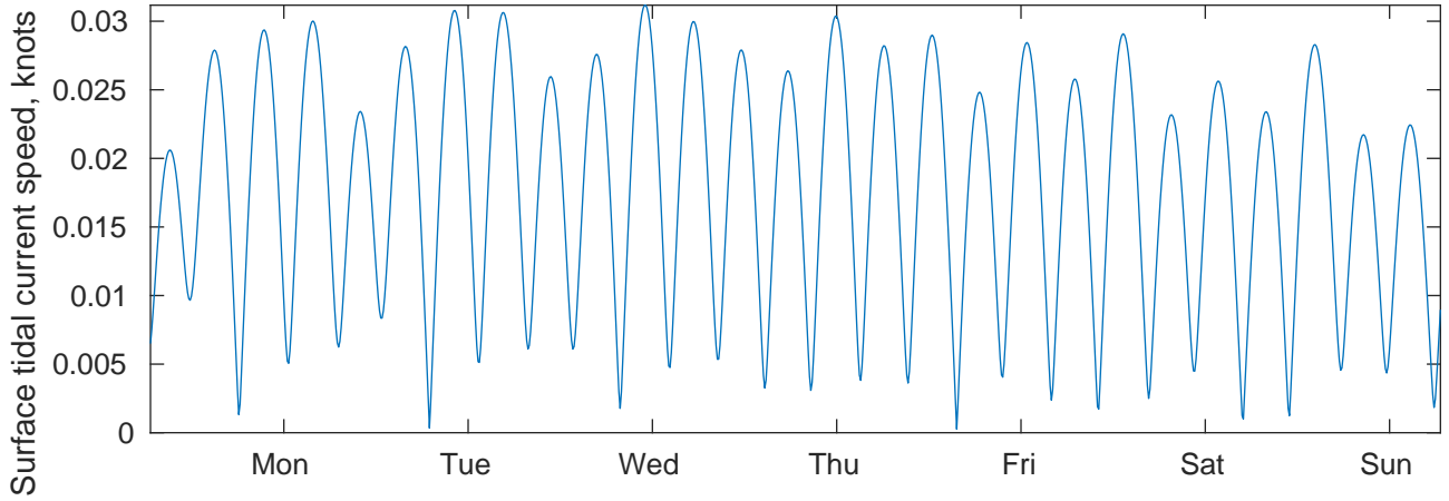
Tidal Currents and Heights for SVP 02 at 20240721
