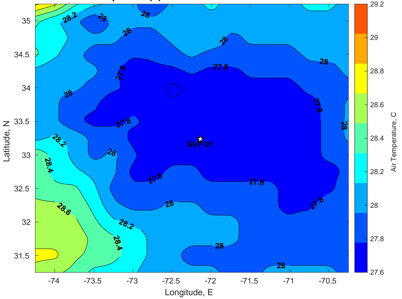
Air Temperature (C) for SVP 01 at 22-Jul-2024
