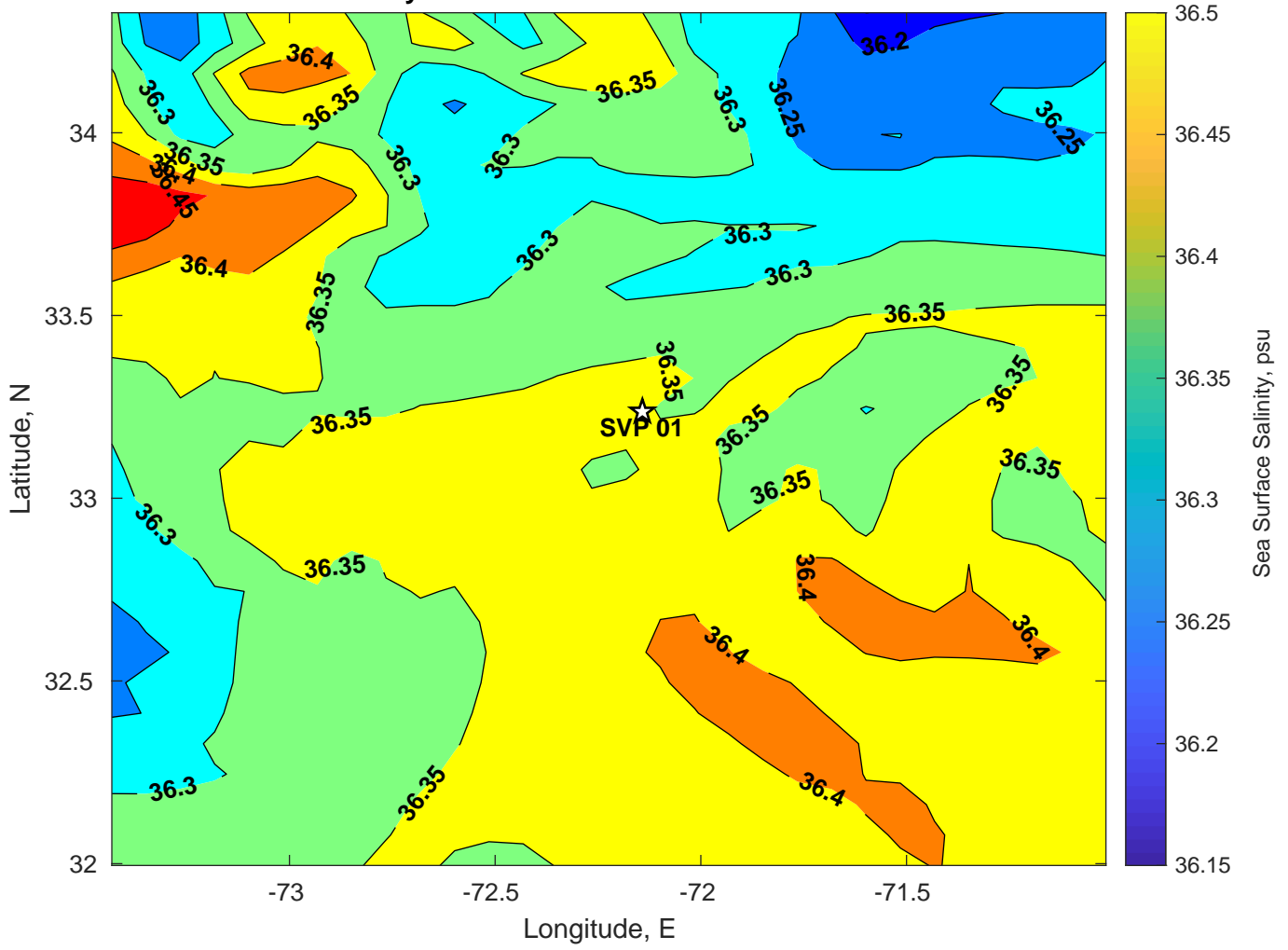
Surface Salinity for SVP 01 at 22-Jul-2024 00:00:00
