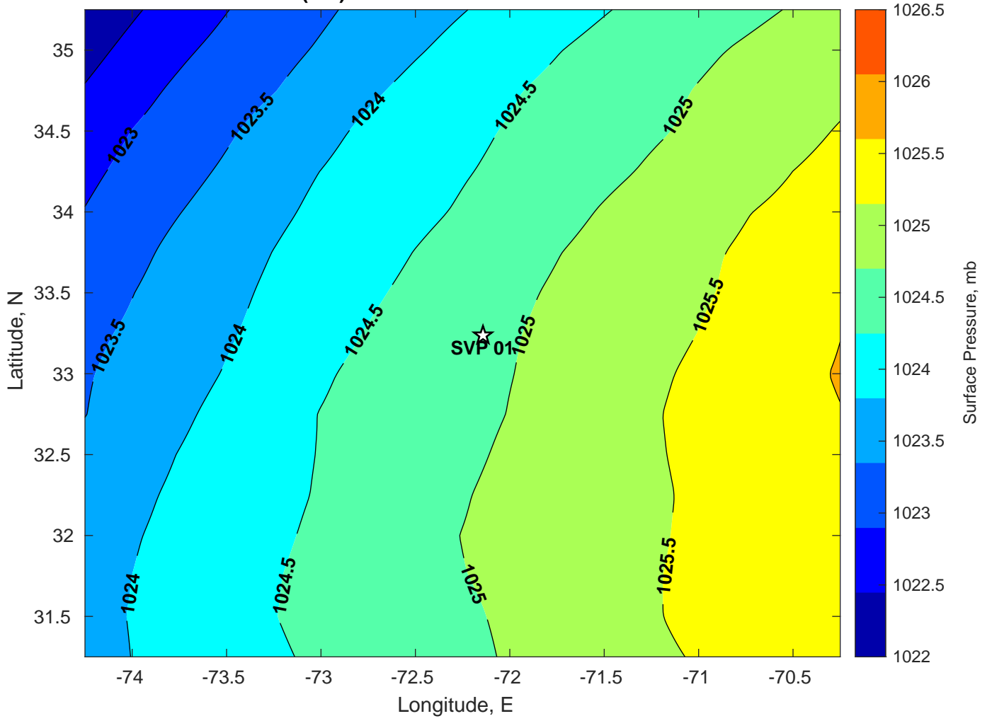
Surface Pressure (mb) for SVP 01 at 24-Jul-2024 00:00:00
