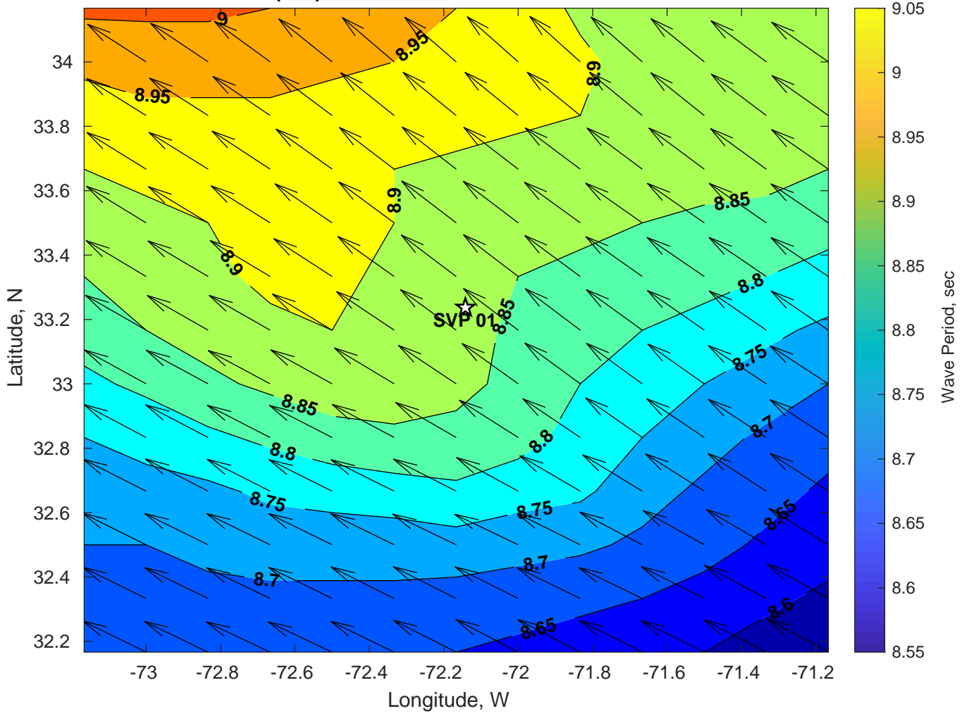
Wave Period (sec) for SVP 01 at 22-Jul-2024 06:00:00
