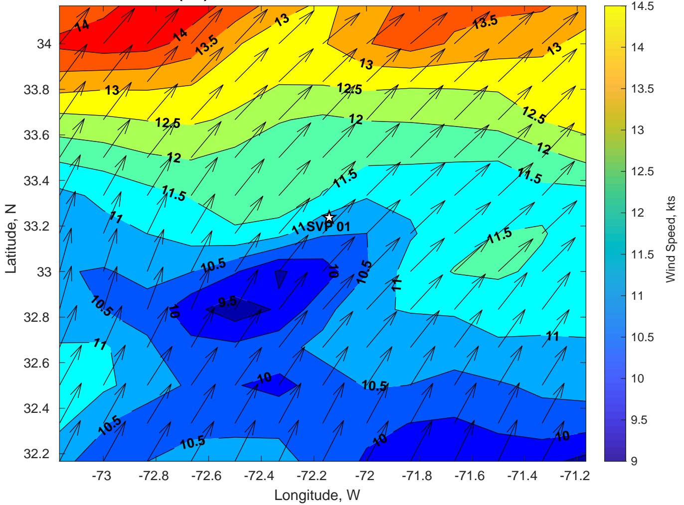
Winds (kts) for SVP 01 at 22-Jul-2024 06:00:00
