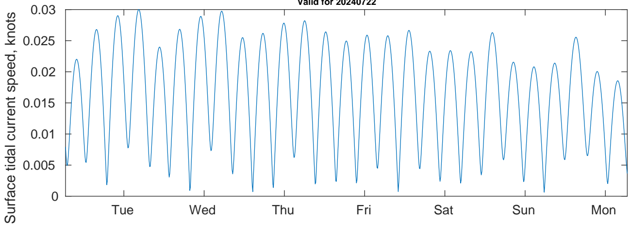
Tidal Currents and Heights for SVP 01 at 20240722
