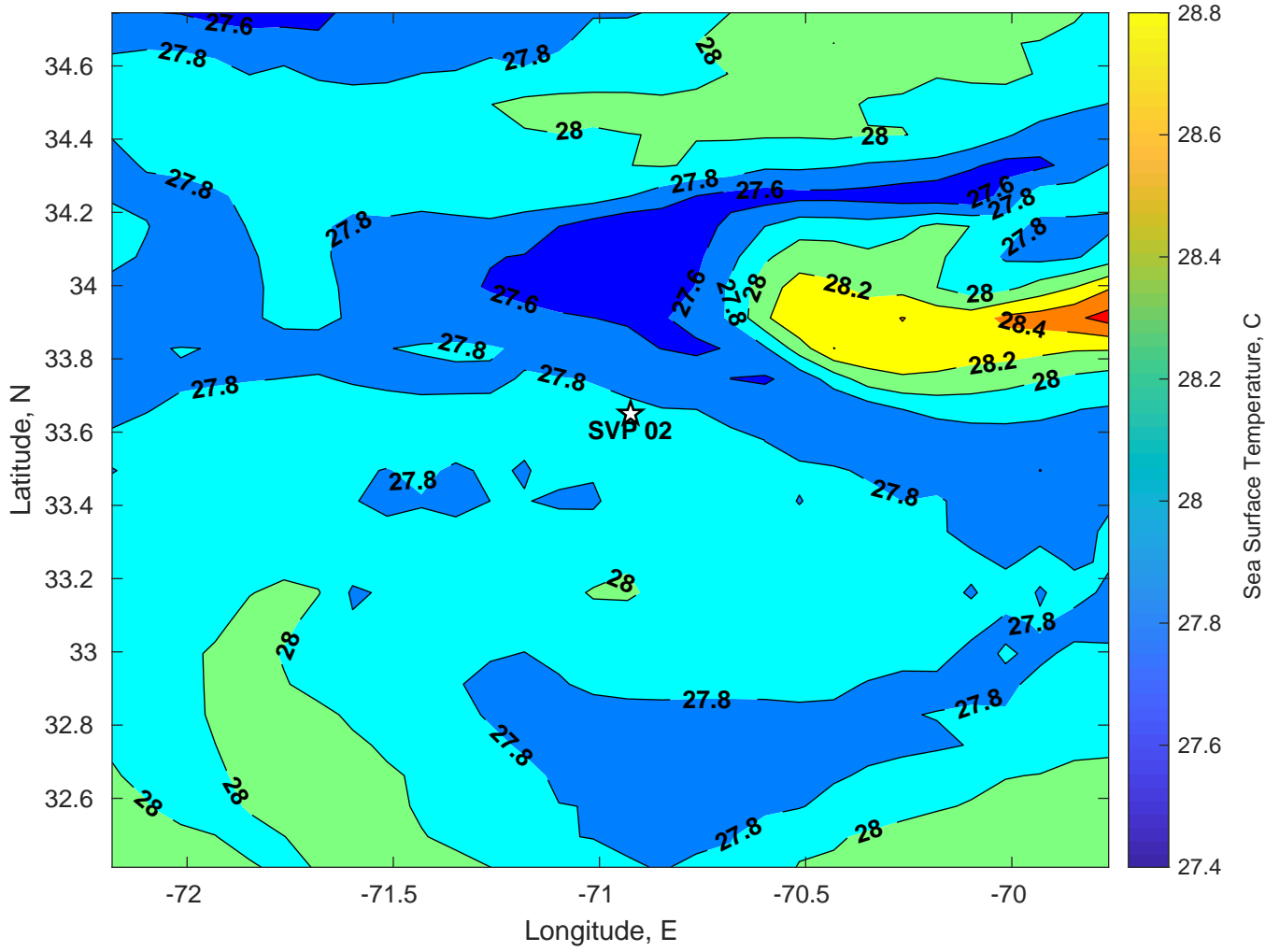
SST for SVP 02 at 22-Jul-2024 00:00:00
