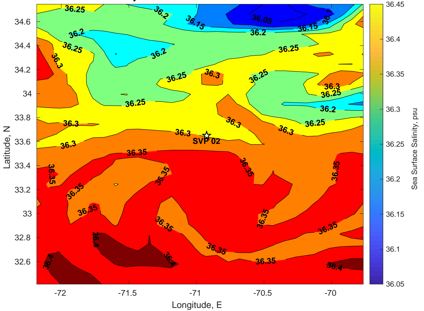
Surface Salinity for SVP 02 at 22-Jul-2024 00:00:00
