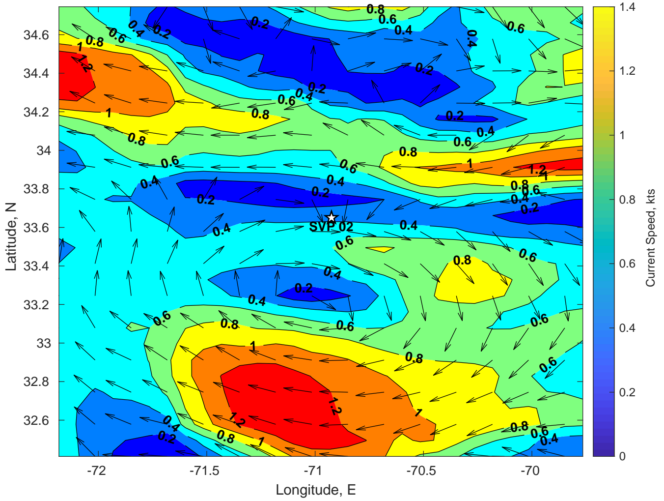
Surface Currents for SVP 02 at 22-Jul-2024 00:00:00
