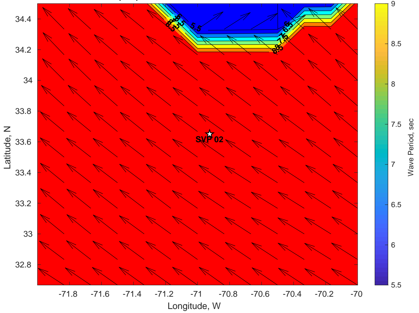
Wave Period (sec) for SVP 02 at 22-Jul-2024 06:00:00
