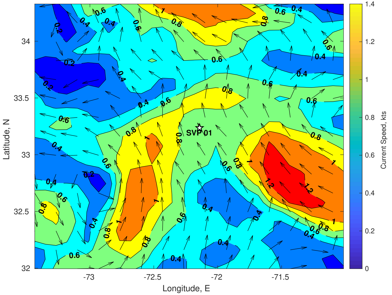
Surface Currents for SVP 01 at 23-Jul-2024 00:00:00
