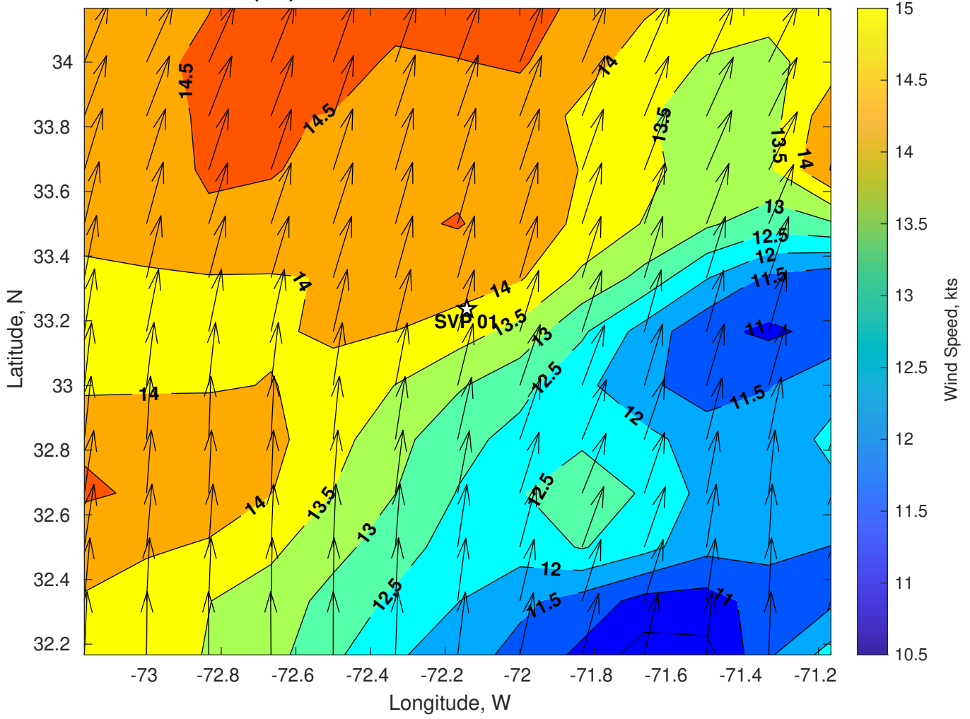
Winds (kts) for SVP 01 at 23-Jul-2024 06:00:00
