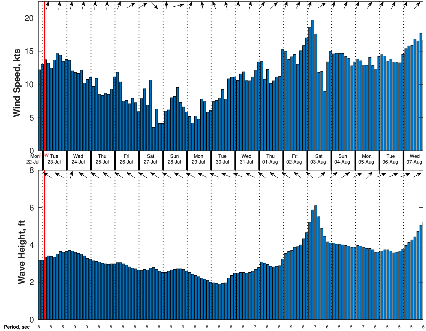
Wind & Wave Forecast for SVP 01 from 22-Jul-2024 19:00:00 to 07-Aug-2024 19:00:00
