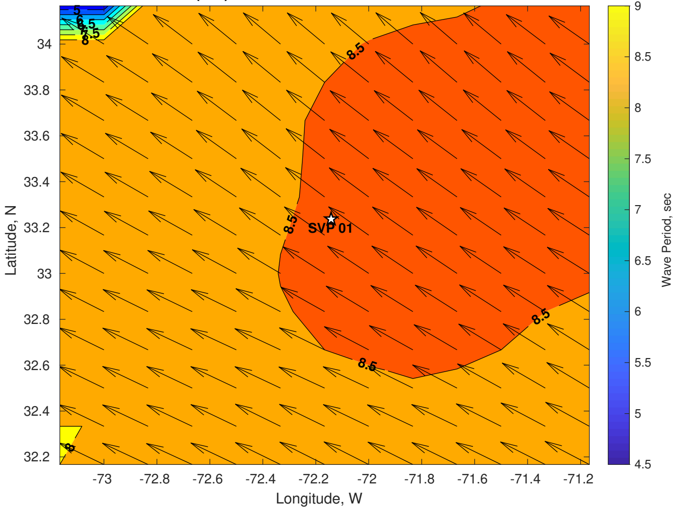
Wave Period (sec) for SVP 01 at 23-Jul-2024 06:00:00
