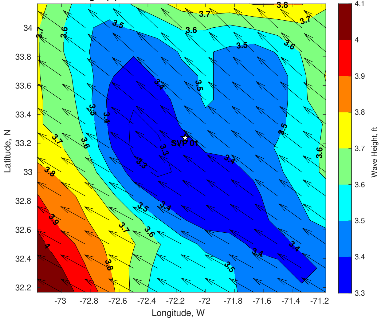
Wave Height (ft) for SVP 01 at 23-Jul-2024 06:00:00
