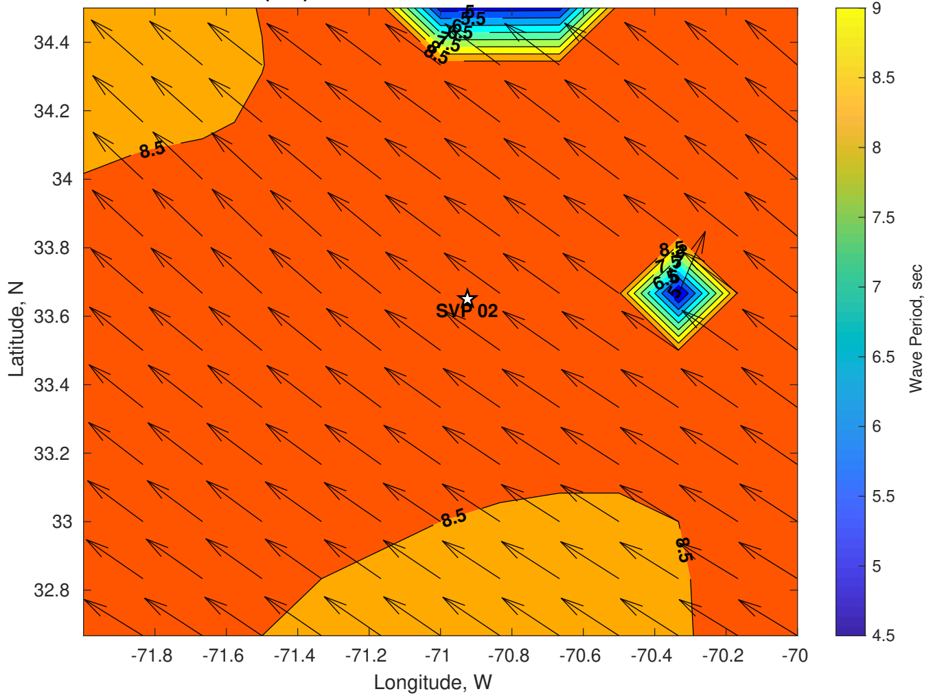
Wave Period (sec) for SVP 02 at 23-Jul-2024 06:00:00
