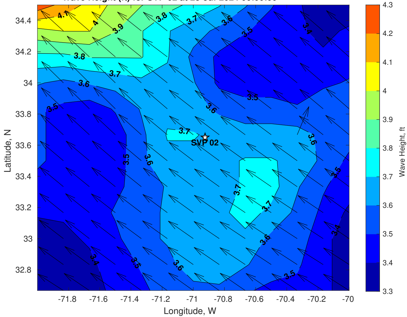
Wave Height (ft) for SVP 02 at 23-Jul-2024 06:00:00
