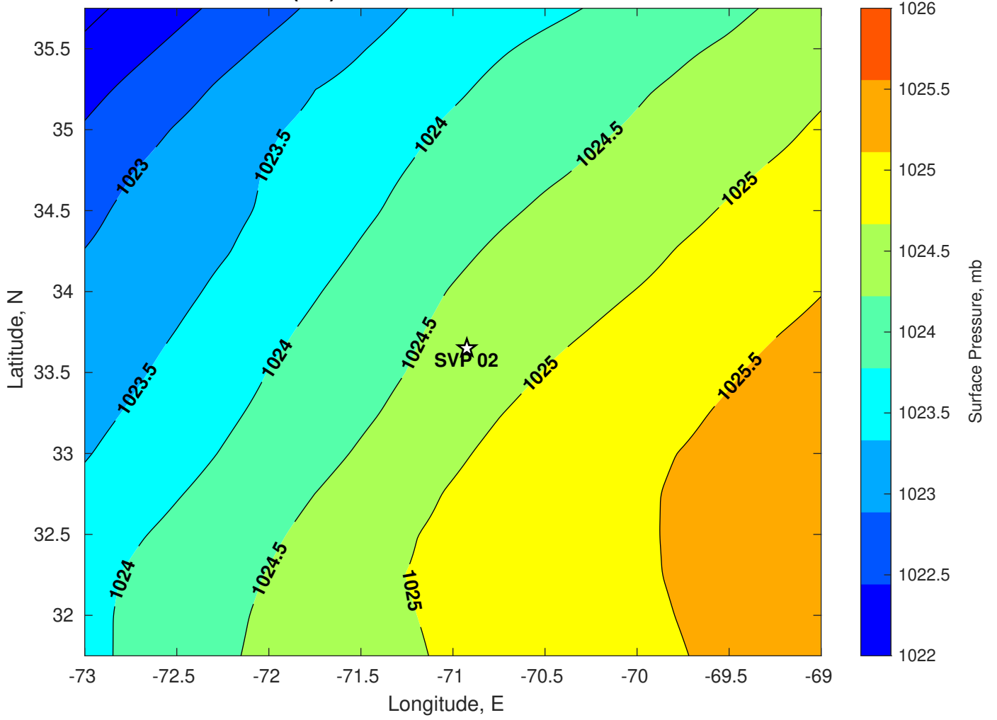
Surface Pressure (mb) for SVP 02 at 24-Jul-2024 00:00:00
