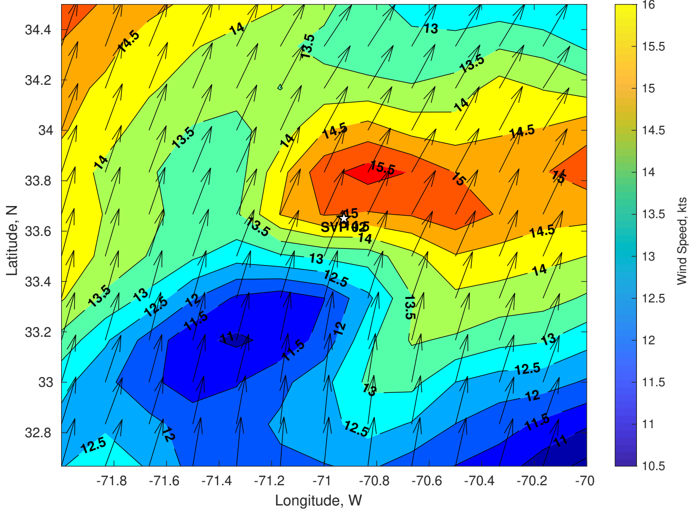
Winds (kts) for SVP 02 at 23-Jul-2024 06:00:00
