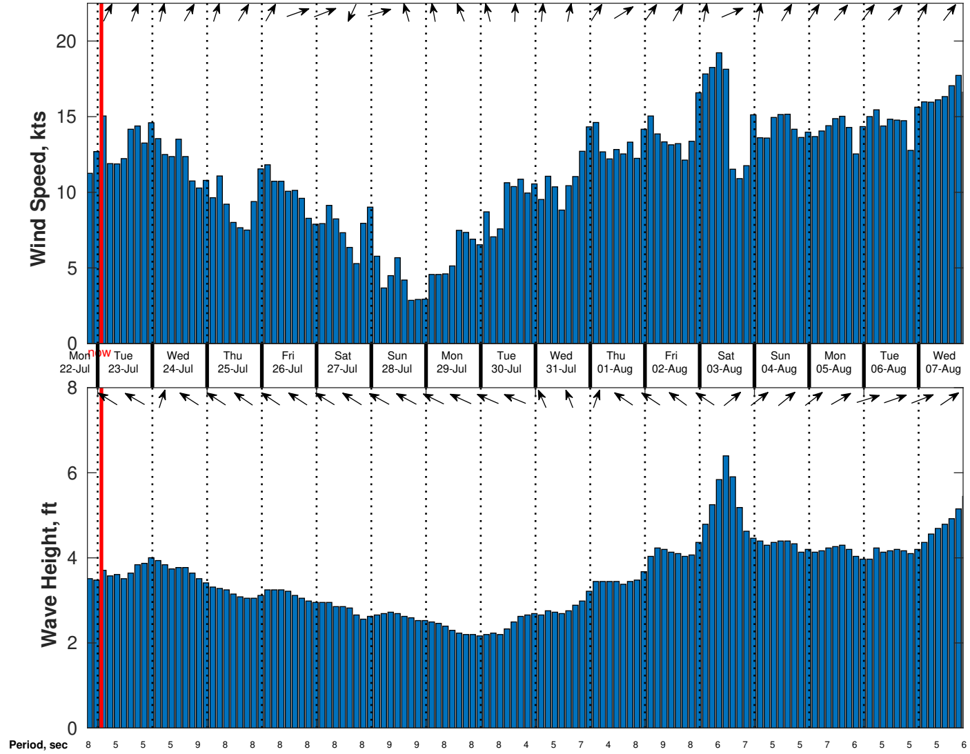
Wind & Wave Forecast for SVP 02 from 22-Jul-2024 19:00:00 to 07-Aug-2024 19:00:00
