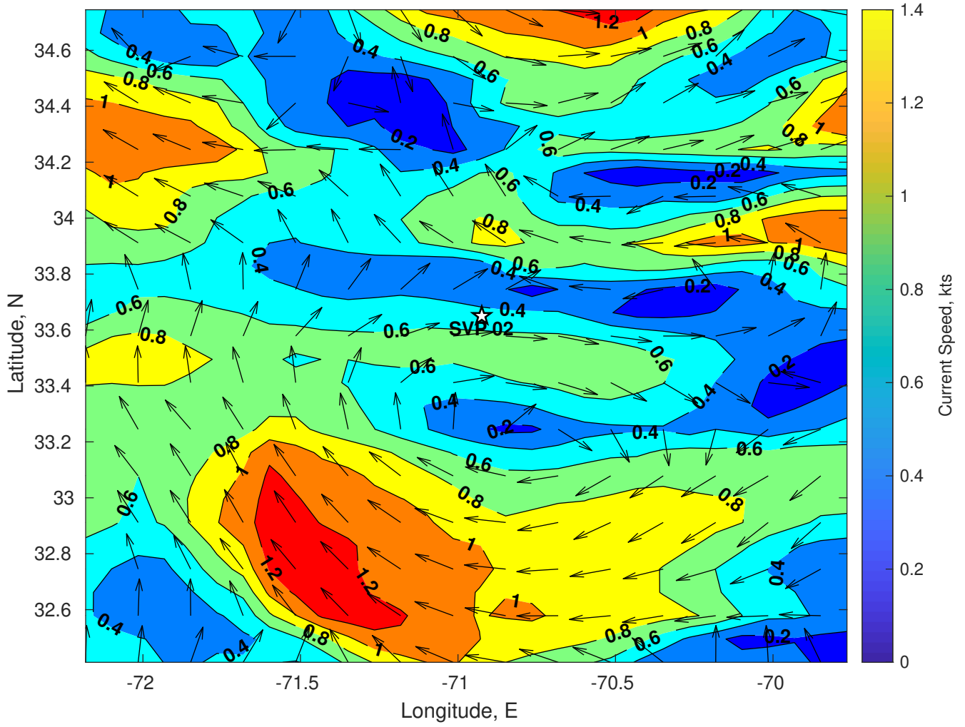
Surface Currents for SVP 02 at 23-Jul-2024 00:00:00
