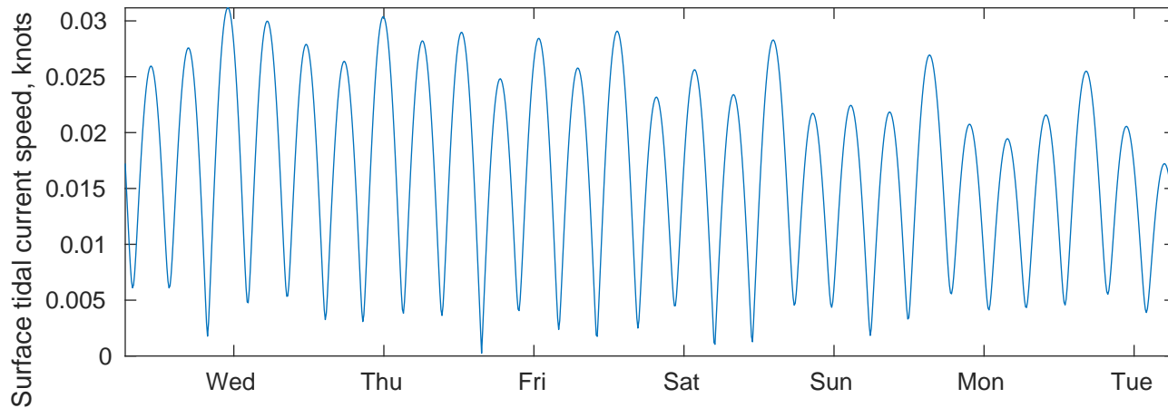
Tidal Currents and Heights for SVP 02 at 20240723
