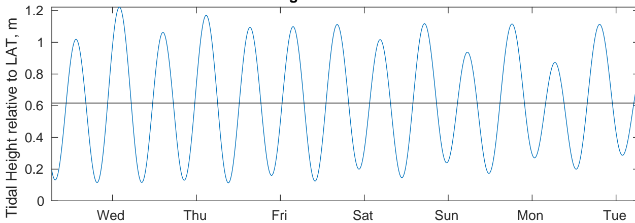
Tidal Currents and Heights for SVP 02 at 20240723
