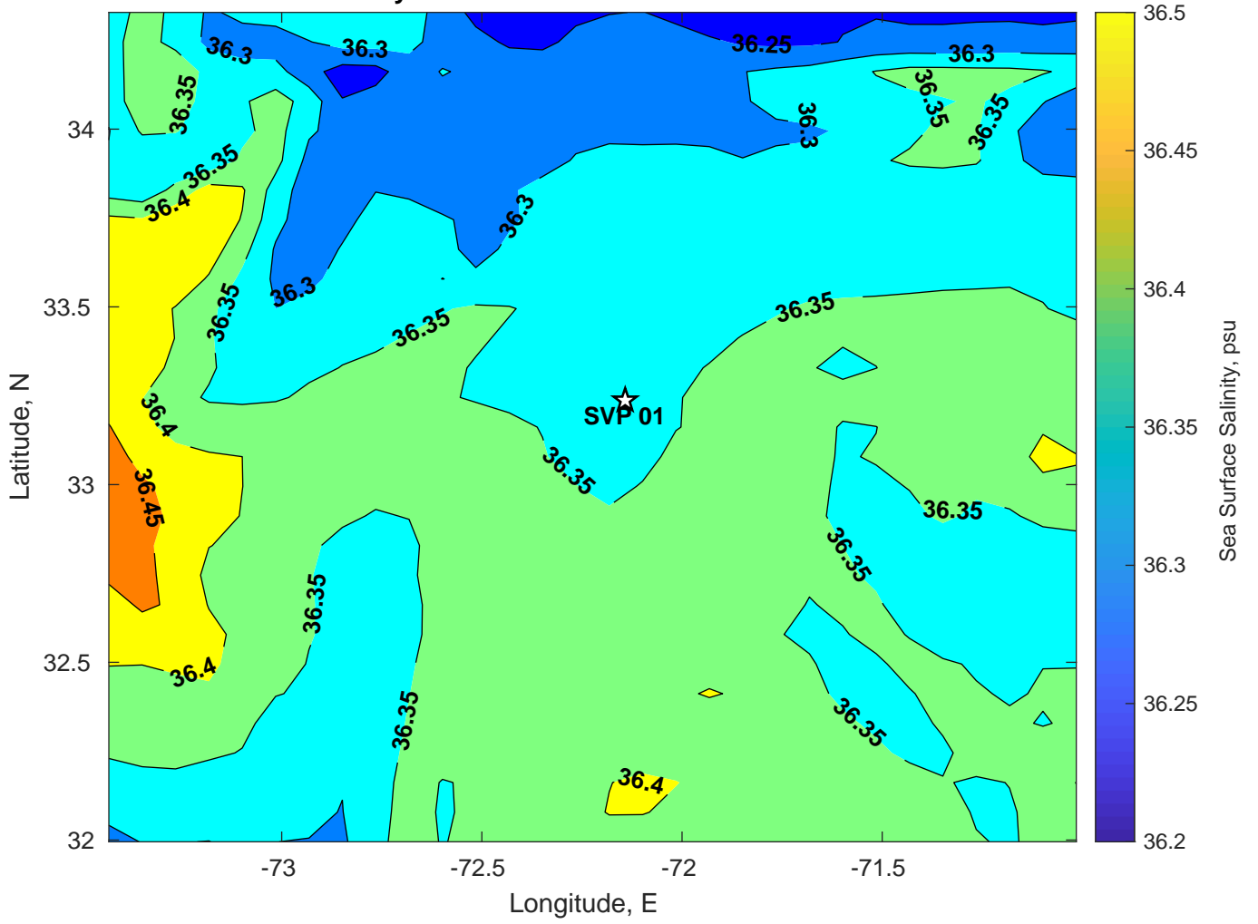
Surface Salinity for SVP 01 at 24-Jul-2024 00:00:00
